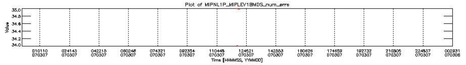
mipas_daily_report_level1_OFI_MIPAS_4_67_P_20070307_28.PNG
