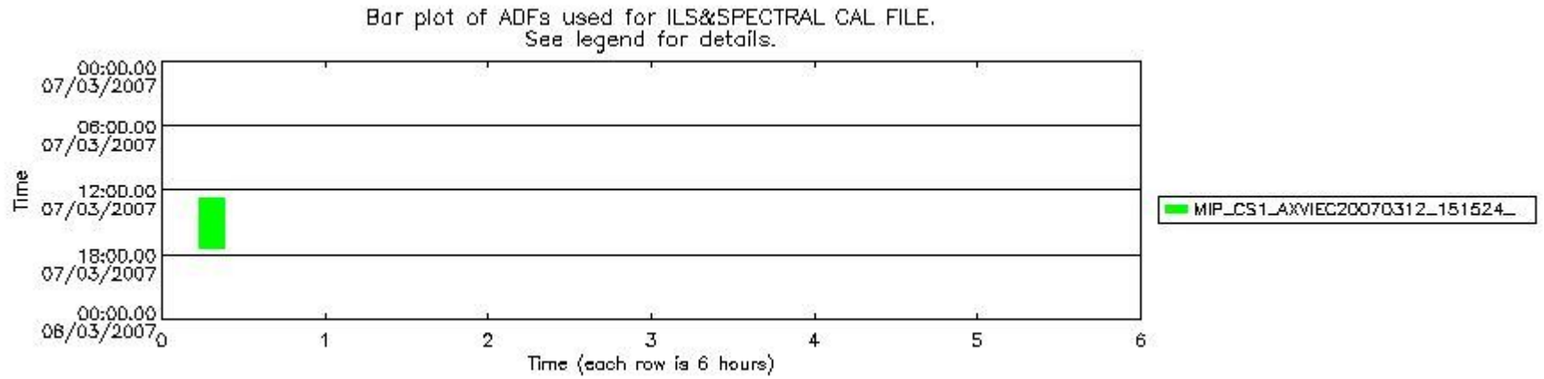
mipas_daily_report_level1_OFL_MIPAS_4_67_P_20070307_53.PNG
