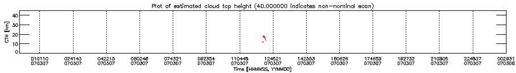
mipas_daily_report_level1_OFL_MIPAS_4_67_P_20070307_51.PNG
