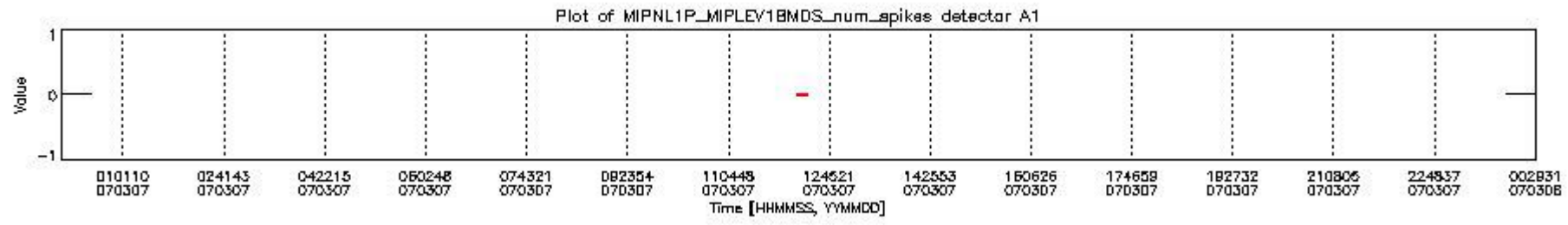
mipas_daily_report_level1_OFL_MIPAS_4_67_P_20070307_16.PNG
