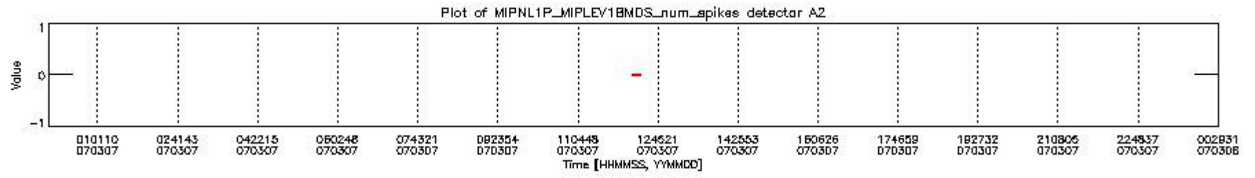
mipas_daily_report_level1_OFI_MIPAS_4_67_P_20070307_18.PNG
