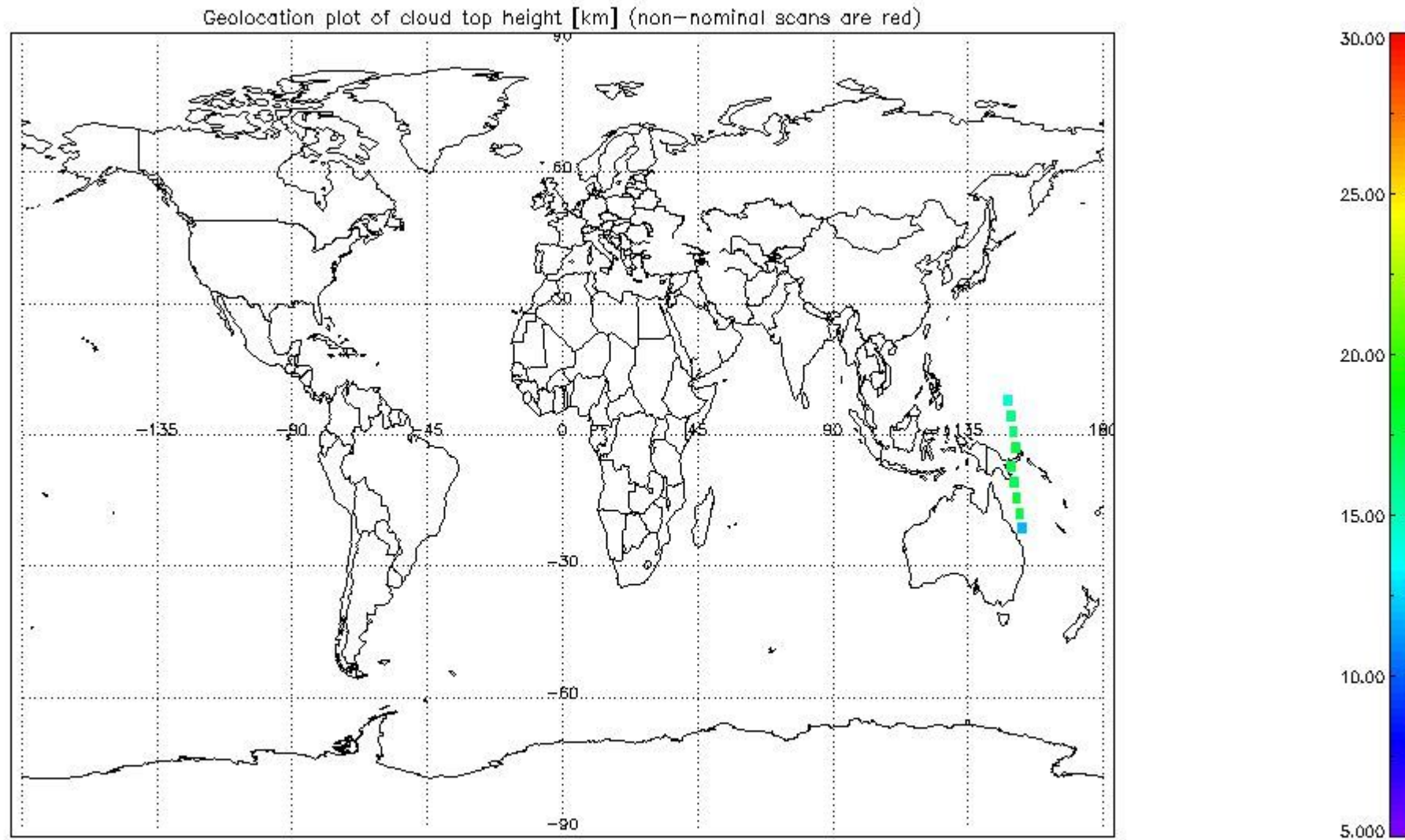
mipas_daily_report_level1_OFL_MIPAS_4_67_P_20070307_51.PNG
