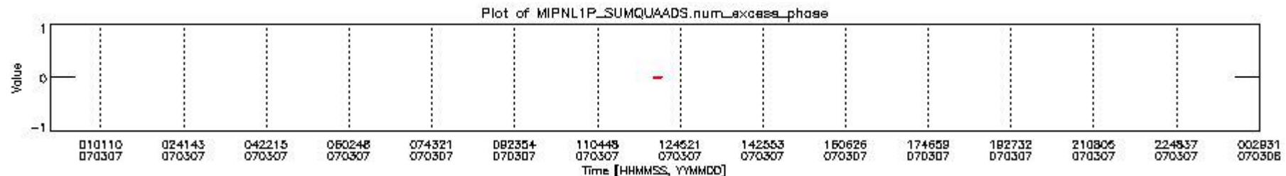
mipas_daily_report_level1_OFI_MIPAS_4_67_P_20070307_8.PNG
