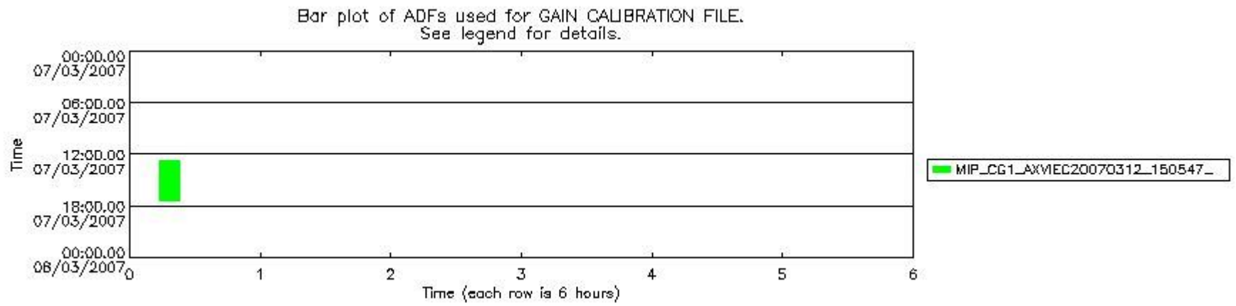
mipas_daily_report_level1_OFL_MIPAS_4_67_P_20070307_54.PNG
