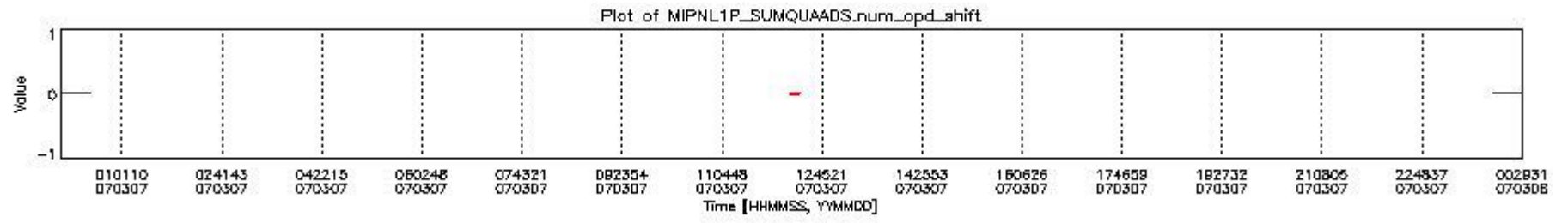
mipas_daily_report_level1_OFL_MIPAS_4_67_P_20070307_10.PNG
