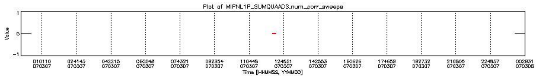
mipas_daily_report_level1_OFI_MIPAS_4_67_P_20070307_2.PNG
