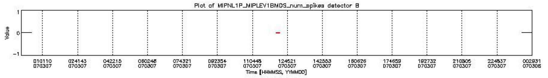
mipas_daily_report_level1_OFI_MIPAS_4_67_P_20070307_22.PNG
