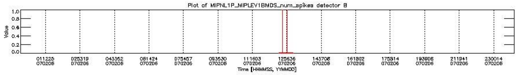
mipas_daily_report_level1_OFI_MIPAS_4_67_P_20070206_22.PNG
