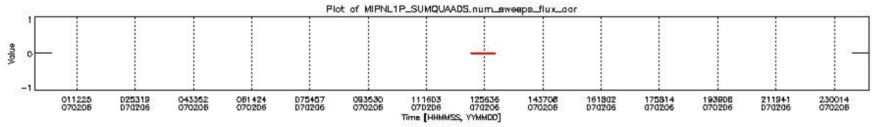
mipas_daily_report_level1_OFI_MIPAS_4_67_P_20070206_12.PNG
