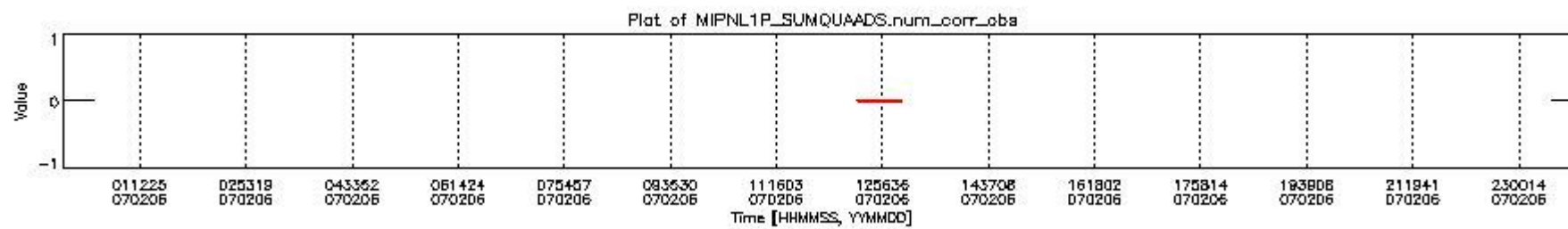
mipas_daily_report_level1_OFI_MIPAS_4_67_P_20070206_6.PNG
