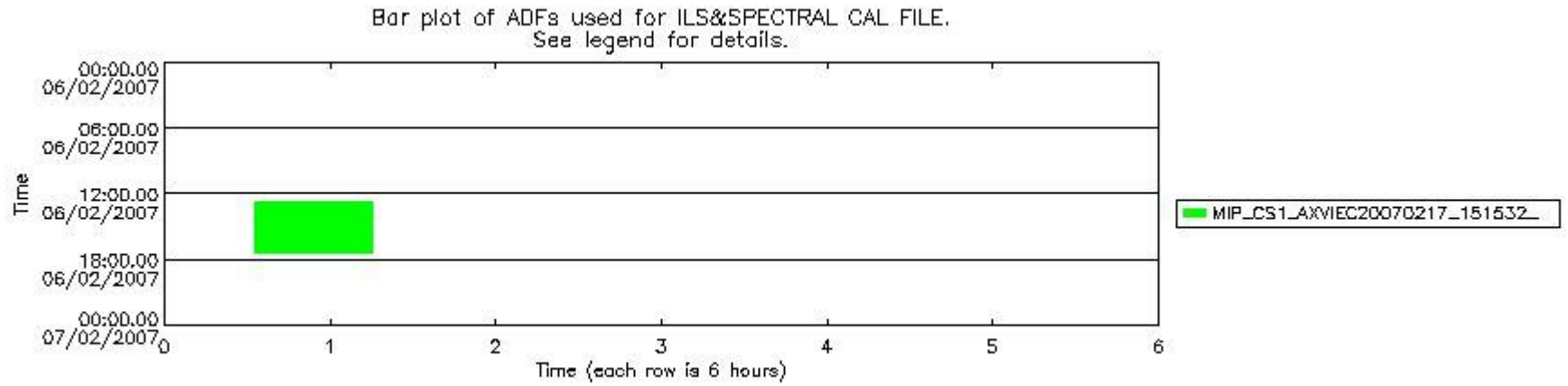
mipas_daily_report_level1_OFI_MIPAS_4_67_P_20070206_53.PNG
