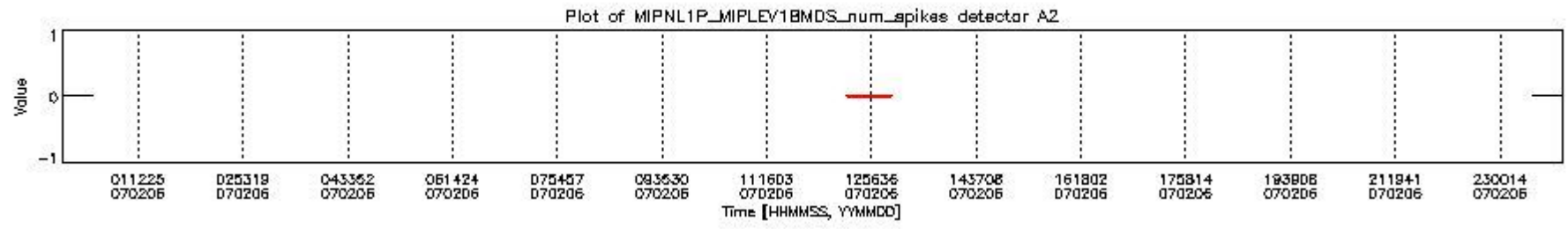
mipas_daily_report_level1_OFI_MIPAS_4_67_P_20070206_18.PNG
