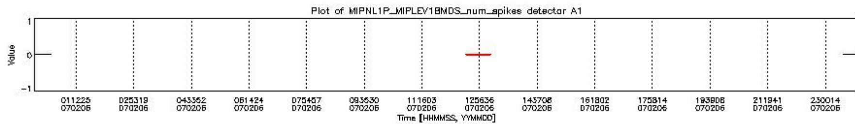
mipas_daily_report_level1_OFL_MIPAS_4_67_P_20070206_16.PNG
