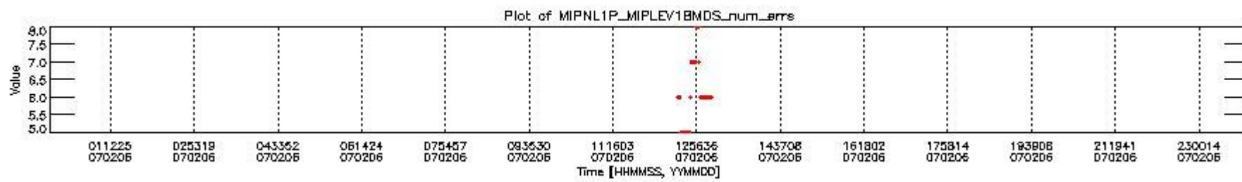
mipas_daily_report_level1_OFI_MIPAS_4_67_P_20070206_28.PNG
