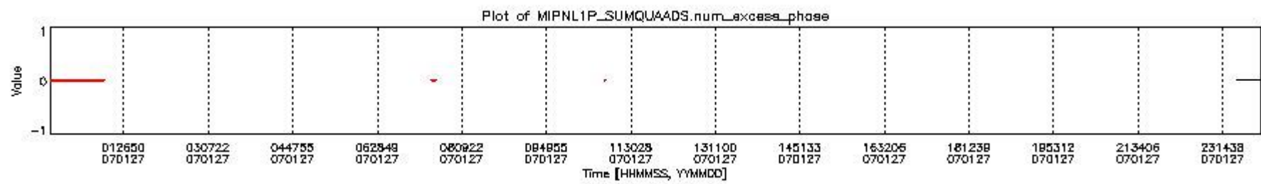
mipas_daily_report_level1_OFI_MIPAS_4_67_P_20070127_8.PNG
