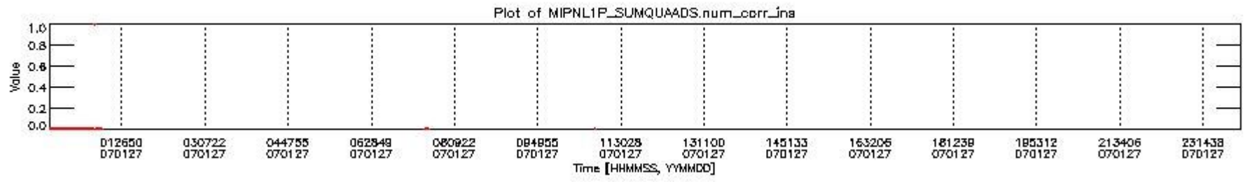
mipas_daily_report_level1_OFI_MIPAS_4_67_P_20070127_4.PNG
