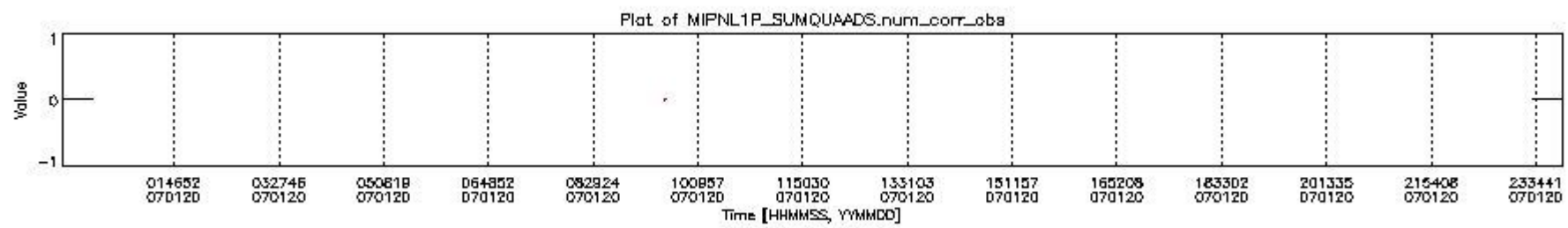
mipas_daily_report_level1_OFI_MIPAS_4_67_P_20070120_6.PNG
