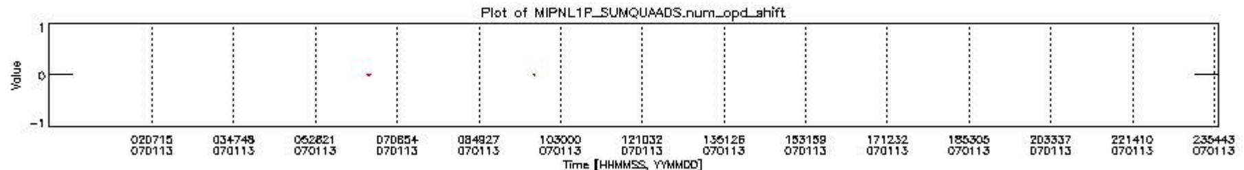
mipas_daily_report_level1_OFI_MIPAS_4_67_P_20070113_10.PNG
