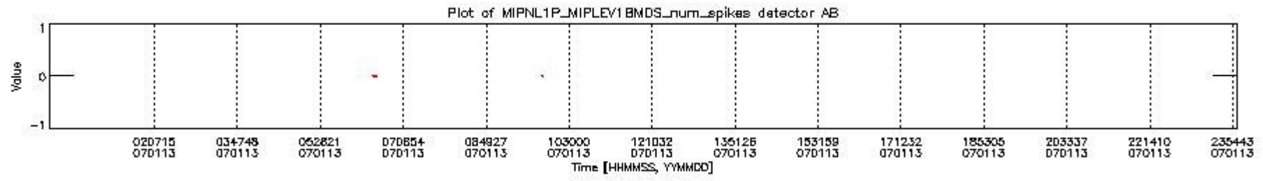
mipas_daily_report_level1_OFI_MIPAS_4_67_P_20070113_20.PNG
