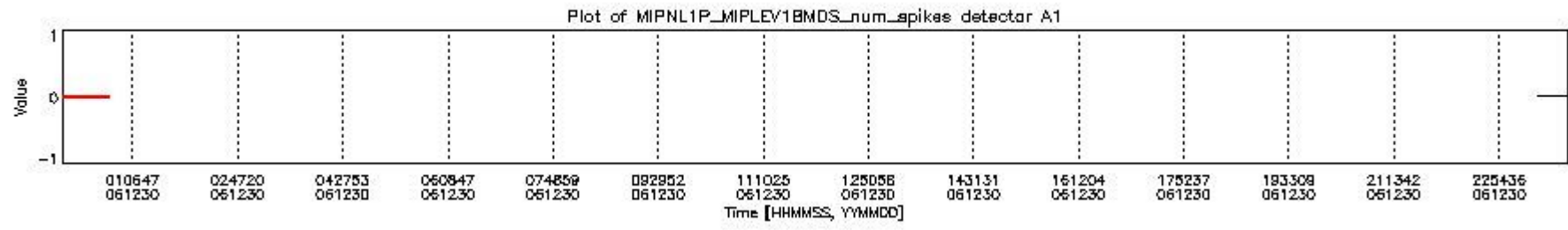
mipas_daily_report_level1_OFL_MIPAS_4_67_P_20061230_16.PNG
