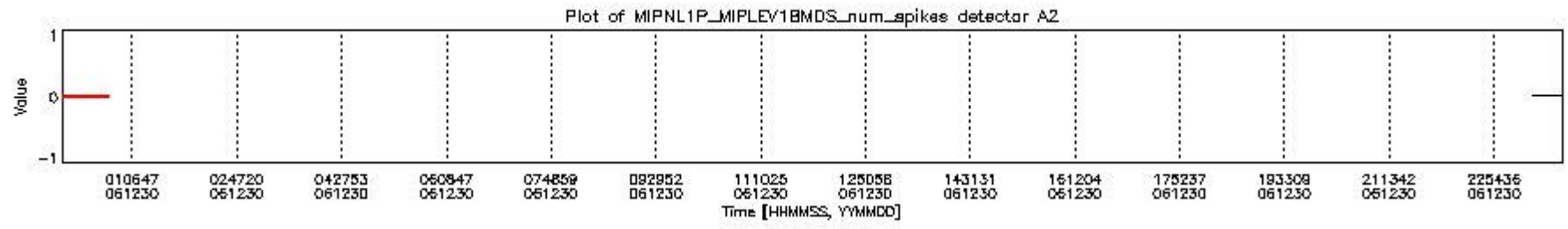
mipas_daily_report_level1_OFI_MIPAS_4_67_P_20061230_18.PNG
