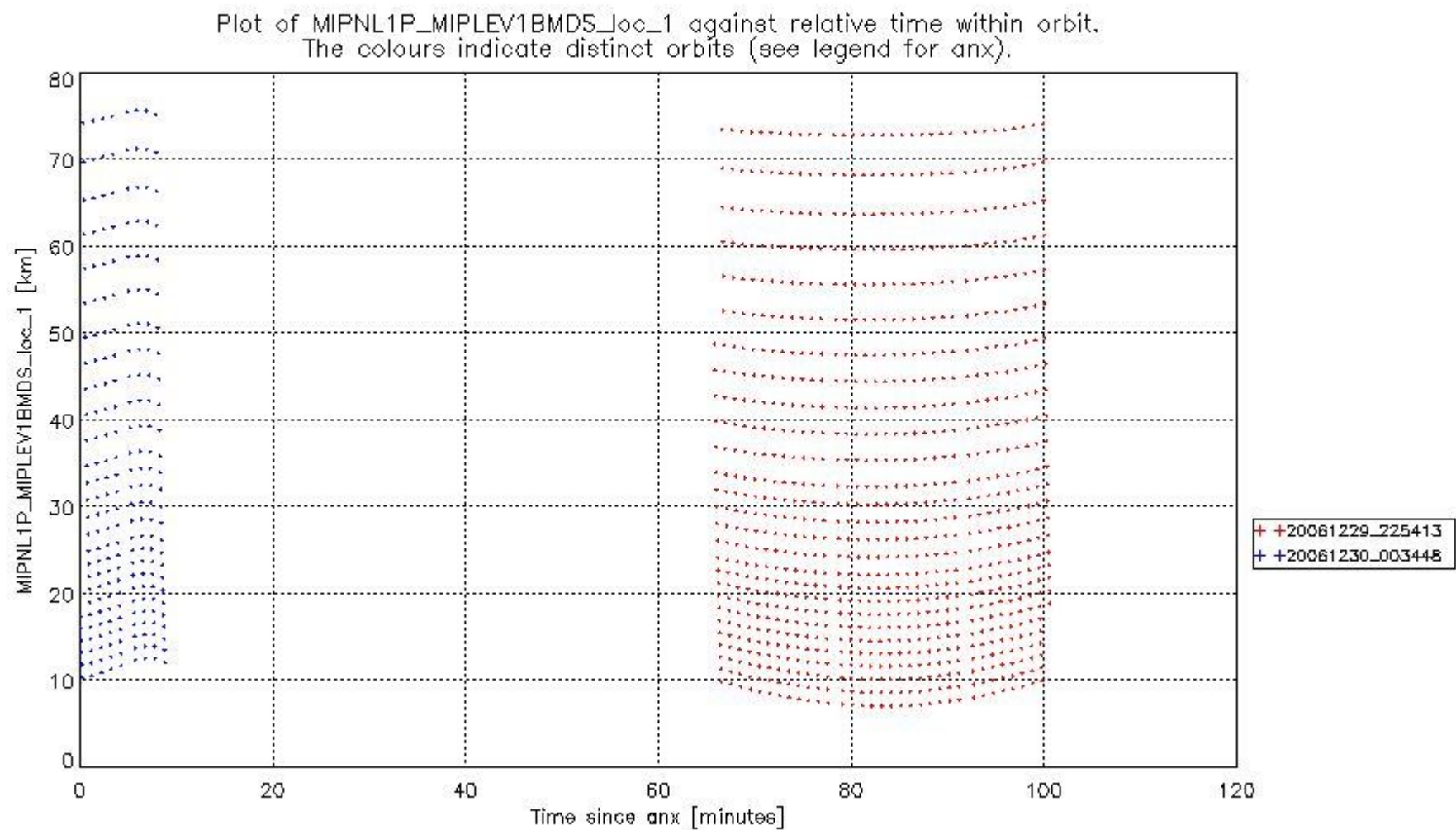
mipas_daily_report_level1_OFL_MIPAS_4_67_P_20061230_50.PNG
