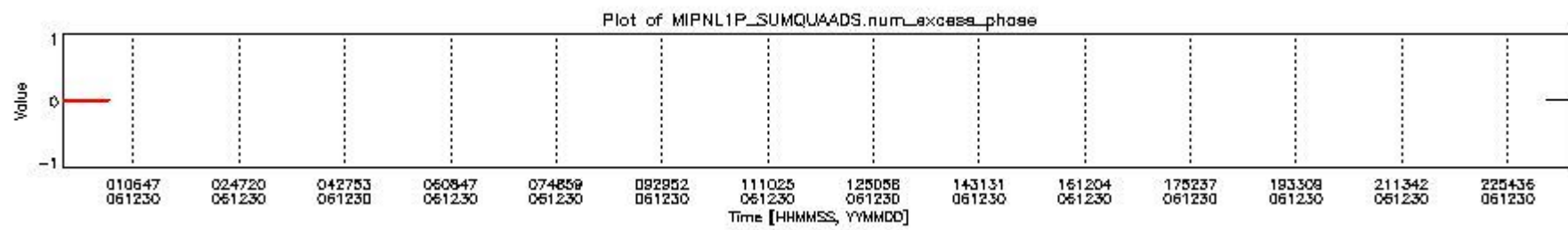
mipas_daily_report_level1_OFI_MIPAS_4_67_P_20061230_8.PNG
