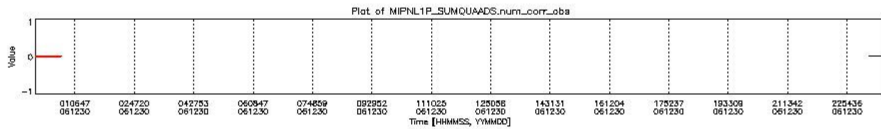
mipas_daily_report_level1_OFI_MIPAS_4_67_P_20061230_6.PNG
