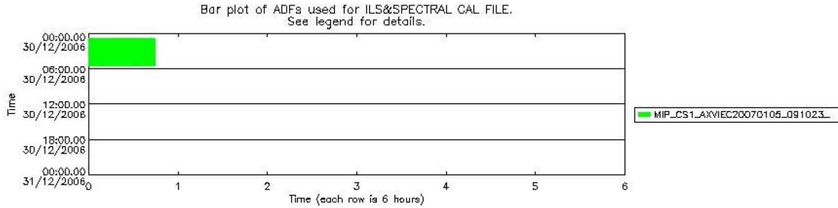
mipas_daily_report_level1_OFL_MIPAS_4_67_P_20061230_53.PNG
