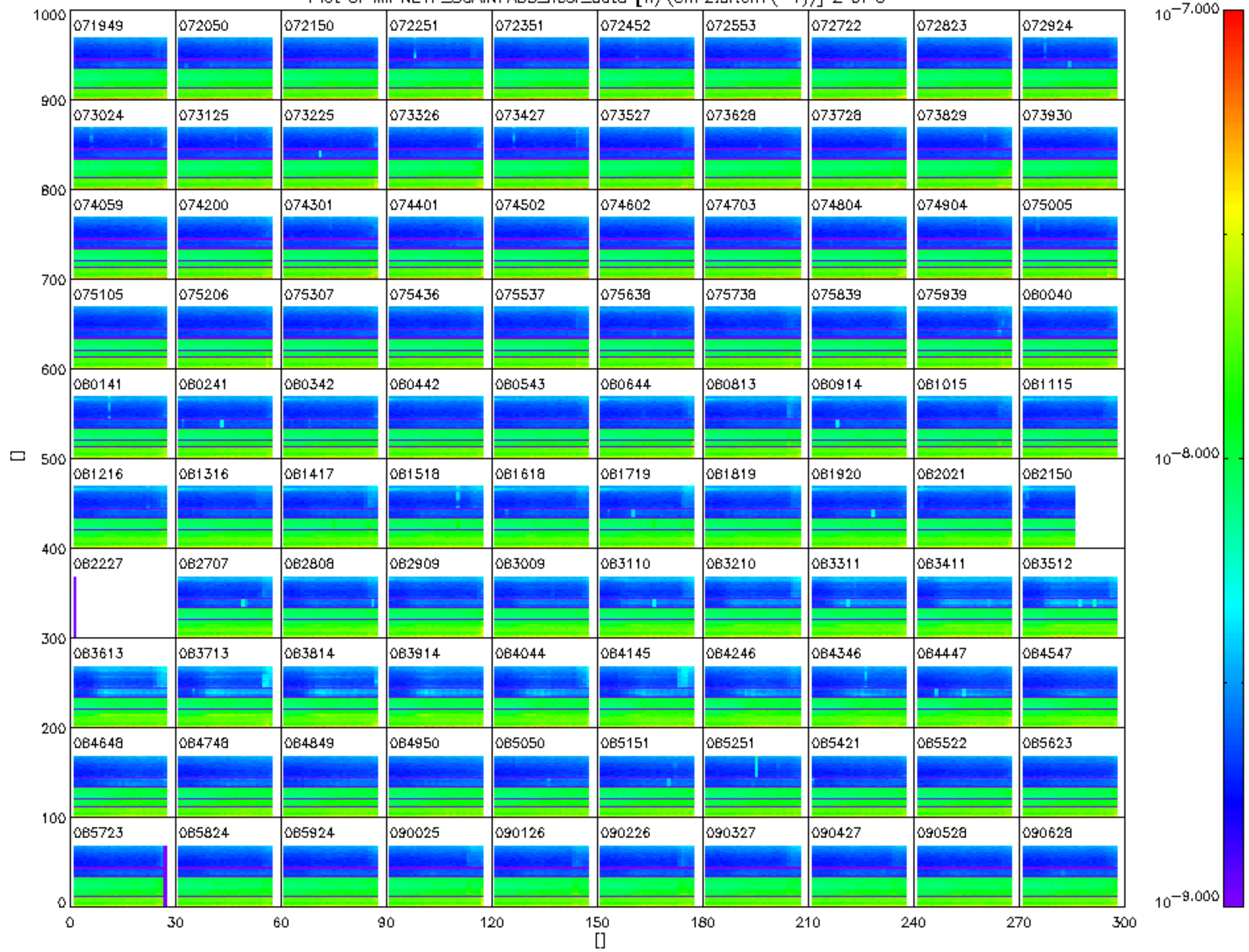
Plot of MIPNL1P_SCAINFADS_nesr_data [W/(cm 2 .sr.cm(-1))] 2 of 5
