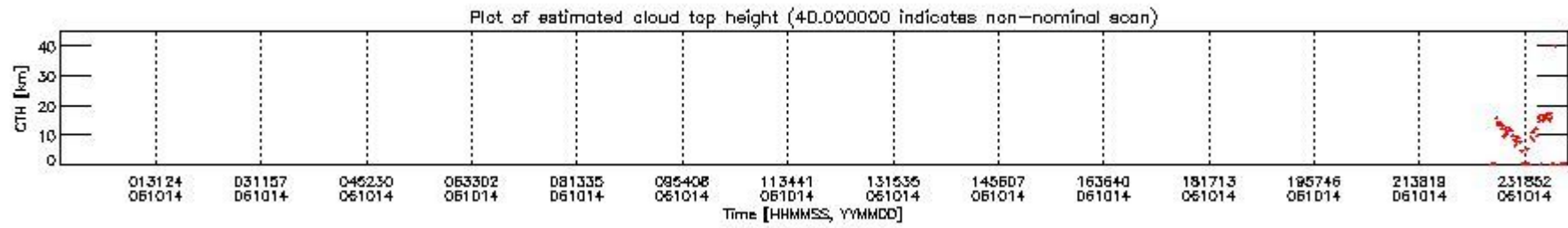
mipas_daily_report_level1_OFL_MIPAS_4_67_P_20061014_51.PNG
