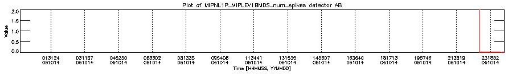
mipas_daily_report_level1_OFI_MIPAS_4_67_P_20061014_20.PNG
