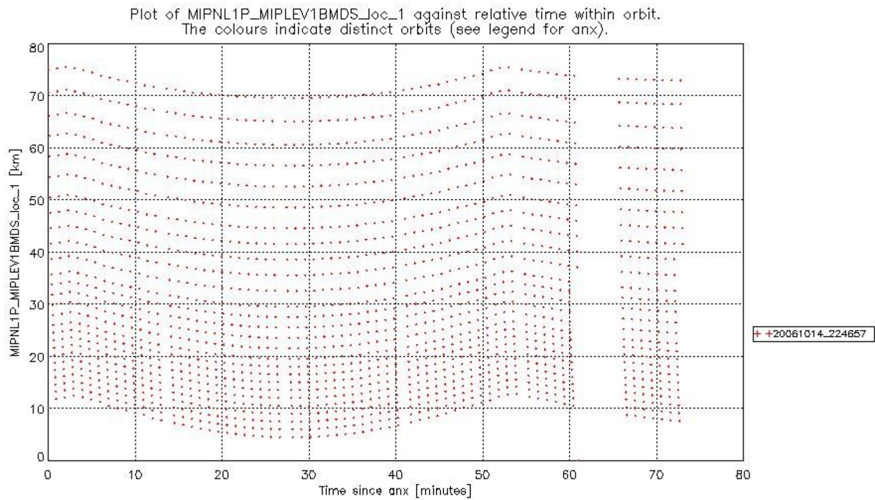
mipas_daily_report_level1_OFL_MIPAS_4_67_P_20061014_50.PNG
