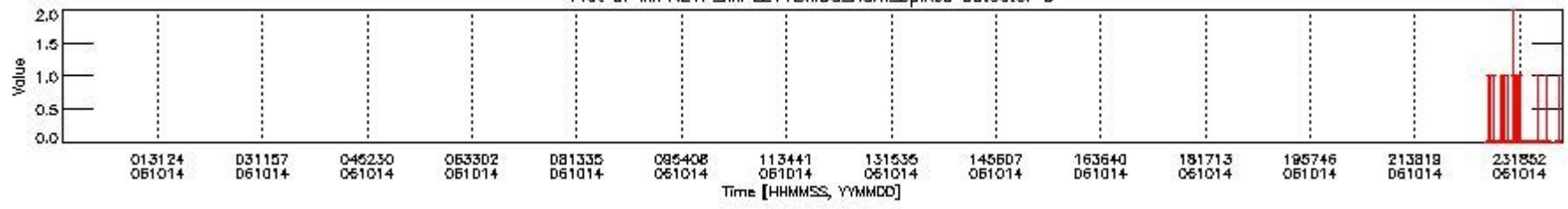
Plot of MIPNL1P_MIPLEV1BMDS_num_spikes detector D
