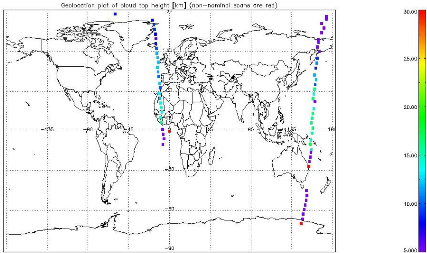
mipas_daily_report_level1_OFL_MIPAS_4_67_P_20061014_51.PNG
