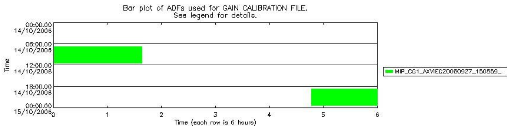
mipas_daily_report_level1_OFL_MIPAS_4_67_P_20061014_54.PNG
