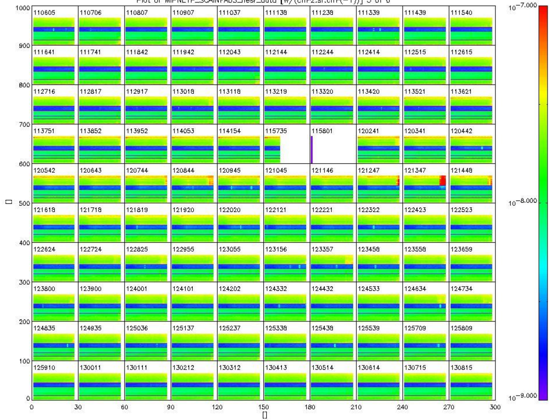
Plot of MIPNL1P_SCAINFADS_nesr_data [W/(cm 2 .sr.cm -1 )] 3 of 6
