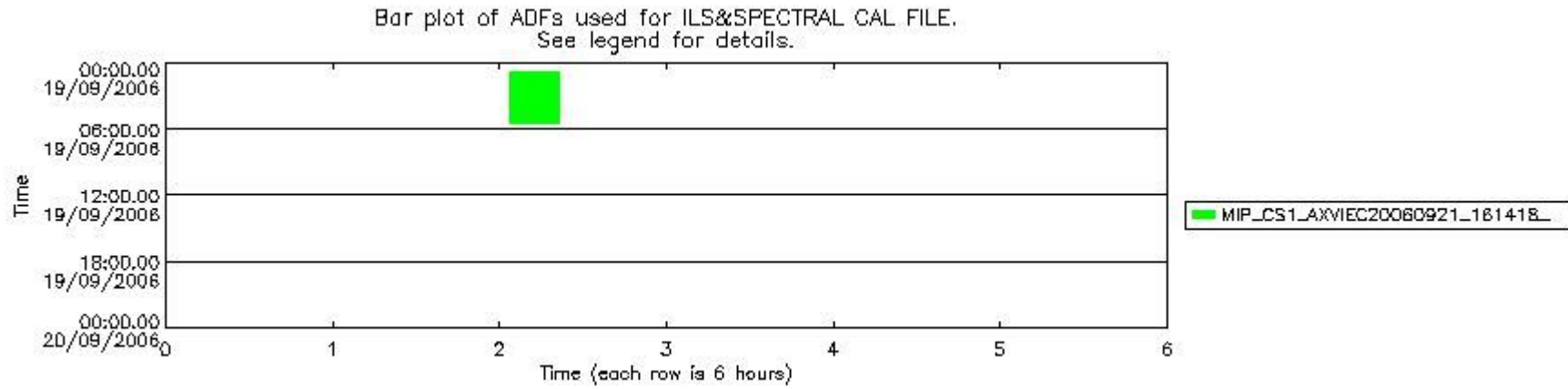
mipas_daily_report_level1_OFL_MIPAS_4_67_P_20060919_53.PNG
