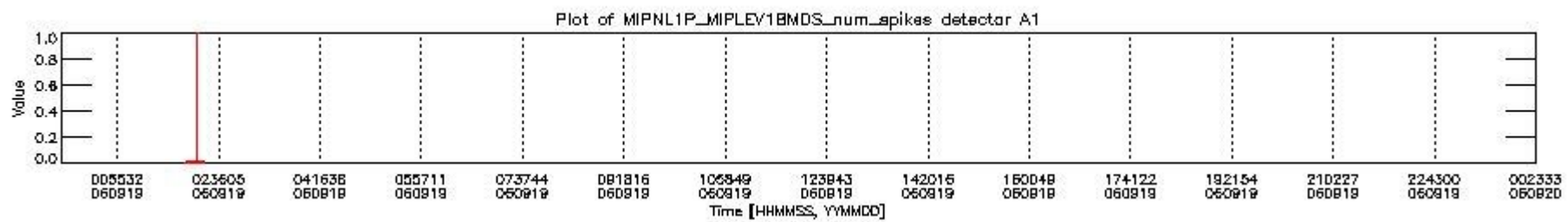
mipas_daily_report_level1_OFL_MIPAS_4_67_P_20060919_16.PNG
