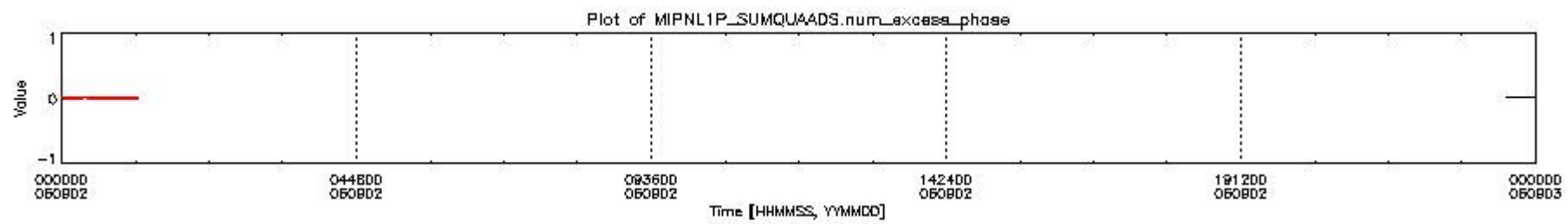
mipas_daily_report_level1_OFI_MIPAS_4_67_P_20060902_8.PNG
