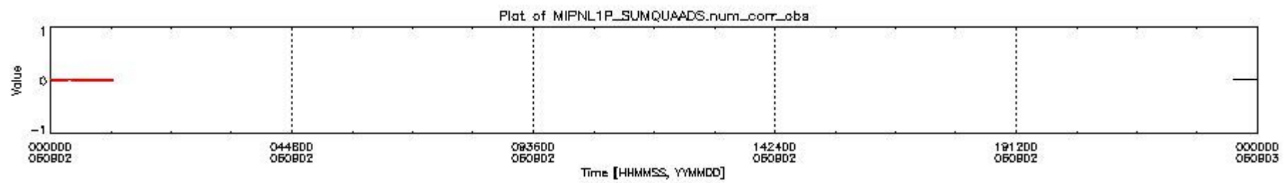
mipas_daily_report_level1_OFI_MIPAS_4_67_P_20060902_6.PNG
