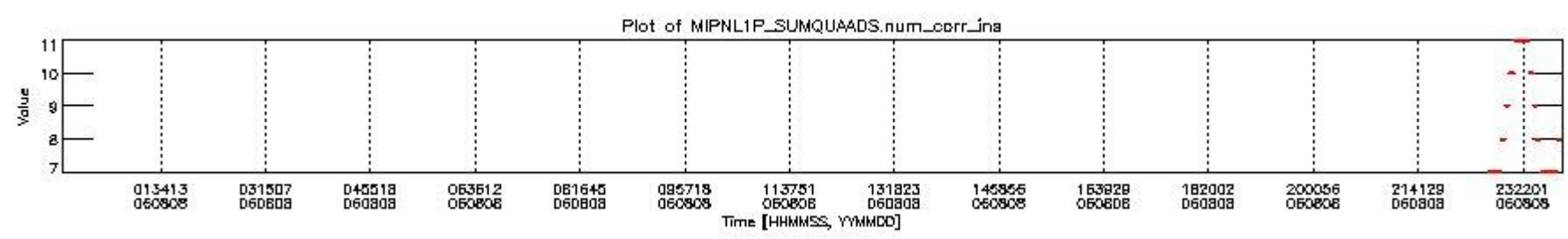
mipas_daily_report_level1_OFI_MIPAS_4_65_P_20060808_4.PNG
