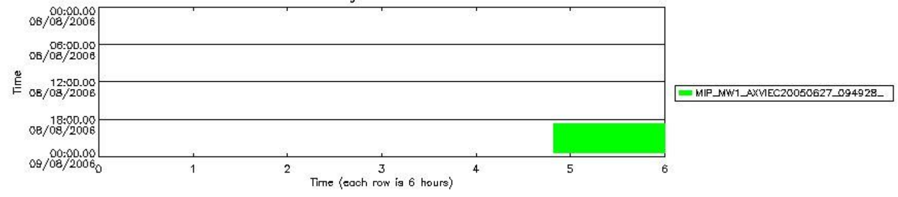
mipas_daily_report_level1_OFL_MIPAS_4_65_P_20060808_58.PNG
