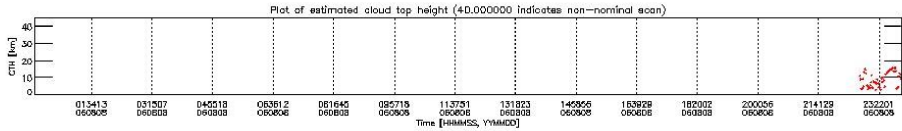
mipas_daily_report_level1_OFL_MIPAS_4_65_P_20060808_51.PNG
