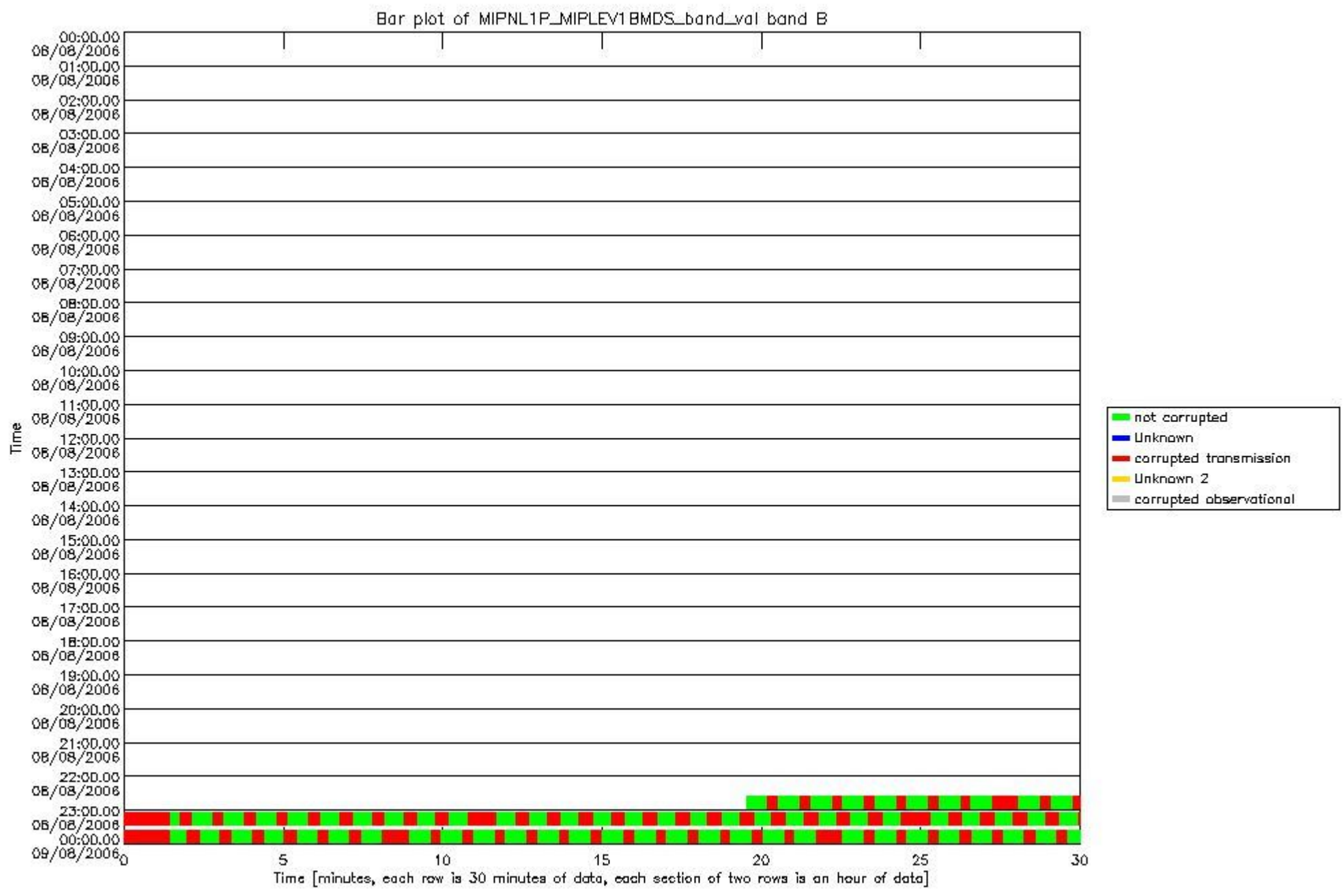
mipas_daily_report_level1_OFI_MIPAS_4_65_P_20060808_34.PNG
