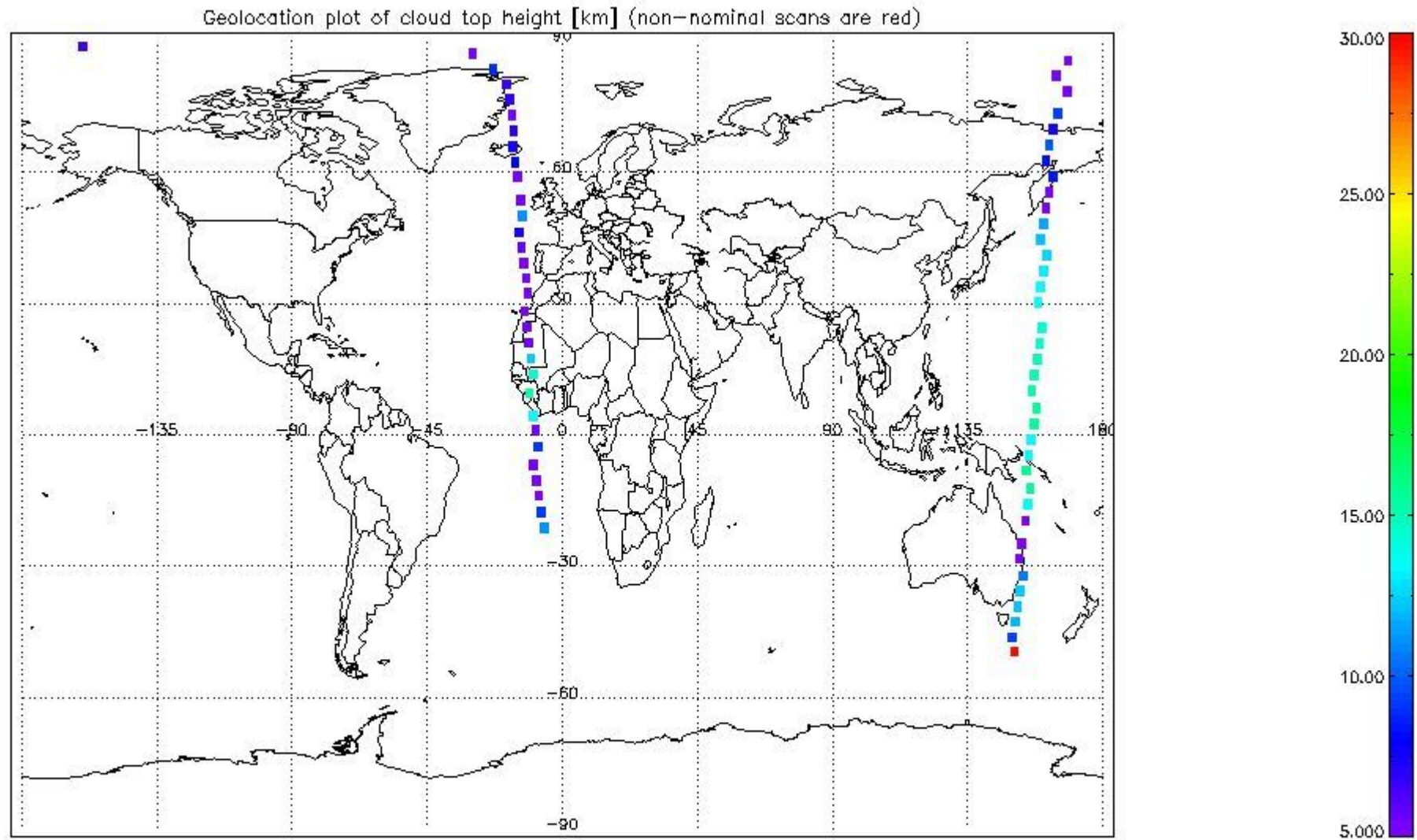
mipas_daily_report_level1_OFL_MIPAS_4_65_P_20060808_51.PNG
