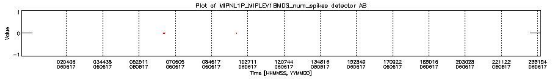
mipas_daily_report_level1_OFI_MIPAS_4_65_P_20060617_20.PNG
