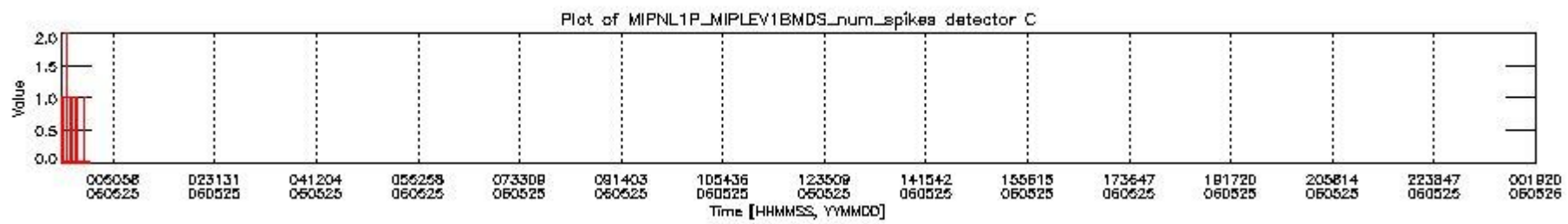
mipas_daily_report_level1_OFI_MIPAS_4_65_P_20060525_24.PNG
