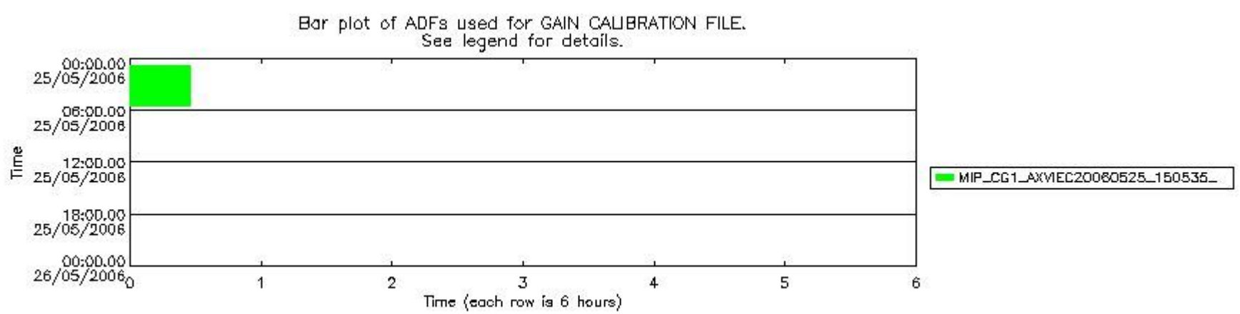
mipas_daily_report_level1_OFI_MIPAS_4_65_P_20060525_52.PNG
