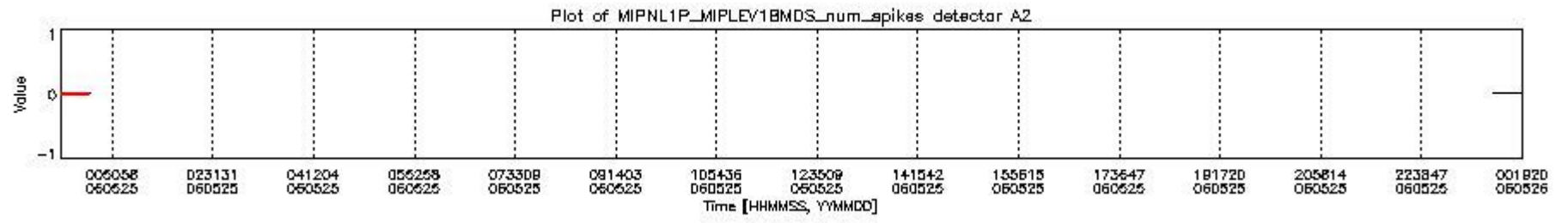
mipas_daily_report_level1_OFI_MIPAS_4_65_P_20060525_18.PNG
