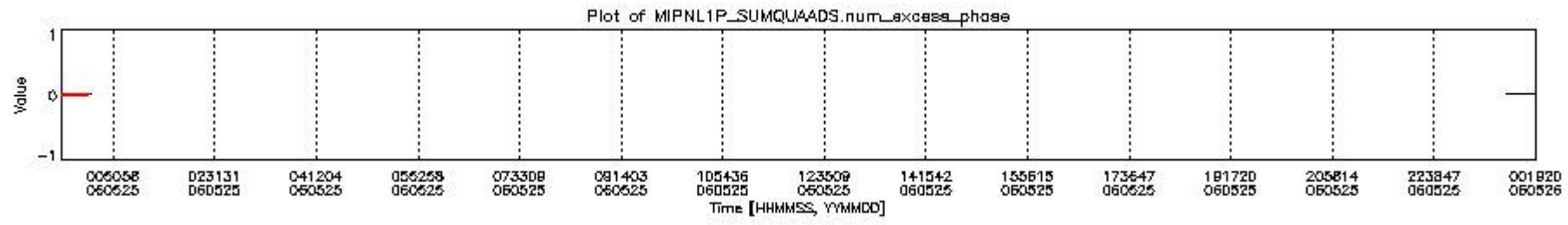
mipas_daily_report_level1_OFI_MIPAS_4_65_P_20060525_8.PNG
