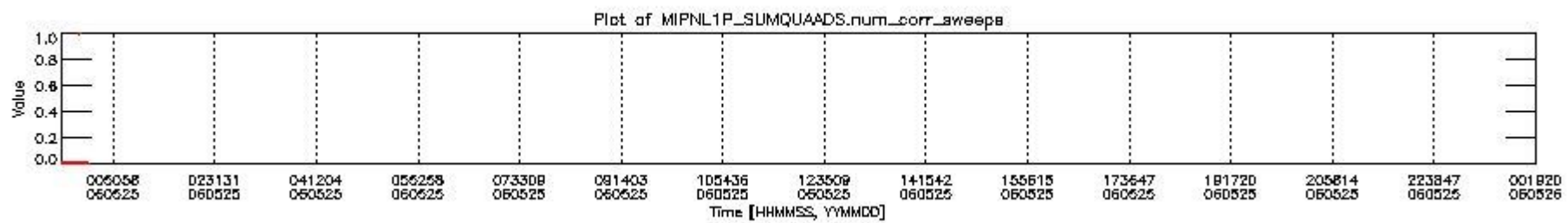
mipas_daily_report_level1_OFI_MIPAS_4_65_P_20060525_2.PNG
