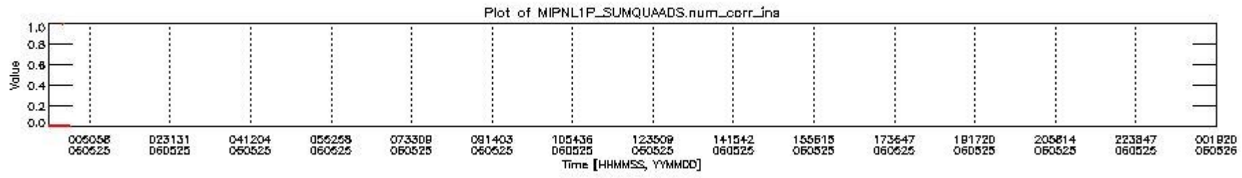
mipas_daily_report_level1_OFI_MIPAS_4_65_P_20060525_4.PNG
