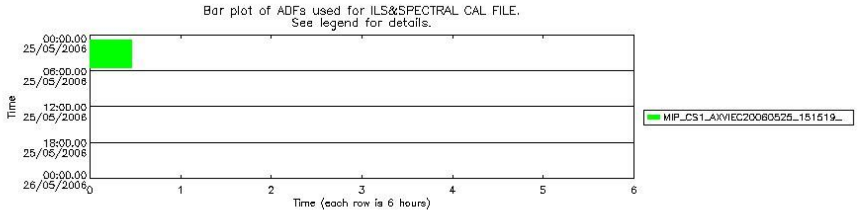
mipas_daily_report_level1_OFI_MIPAS_4_65_P_20060525_51.PNG
