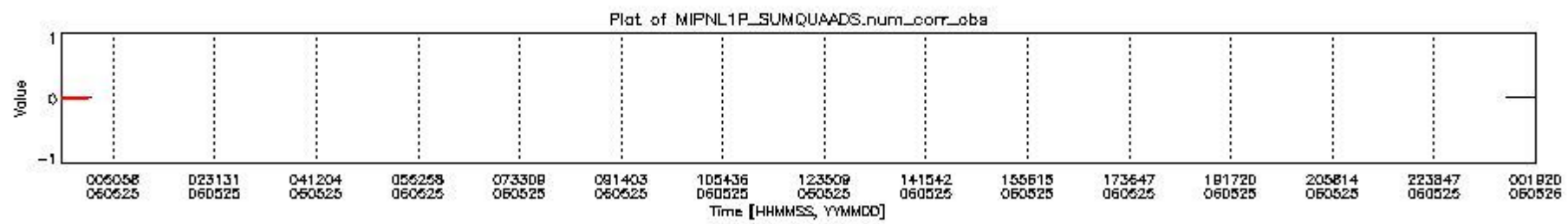
mipas_daily_report_level1_OFI_MIPAS_4_65_P_20060525_6.PNG
