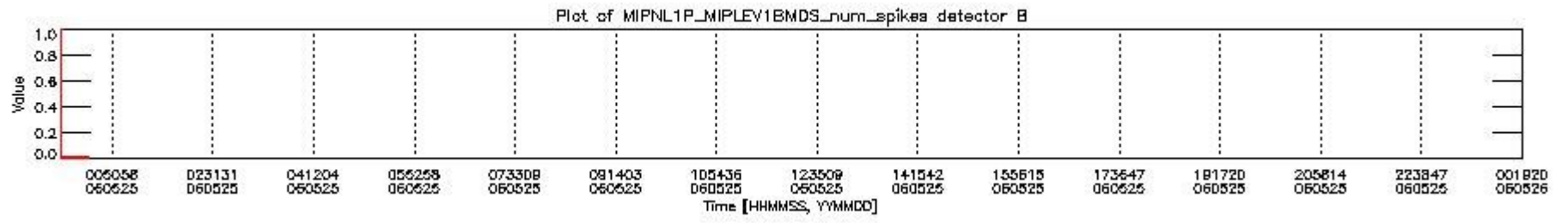
mipas_daily_report_level1_OFI_MIPAS_4_65_P_20060525_22.PNG
