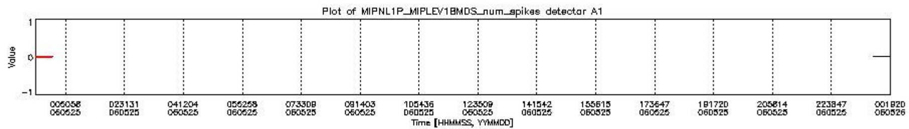
mipas_daily_report_level1_OFL_MIPAS_4_65_P_20060525_16.PNG
