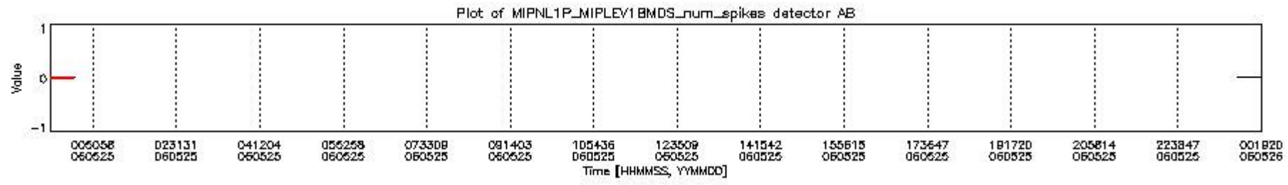
mipas_daily_report_level1_OFI_MIPAS_4_65_P_20060525_20.PNG
