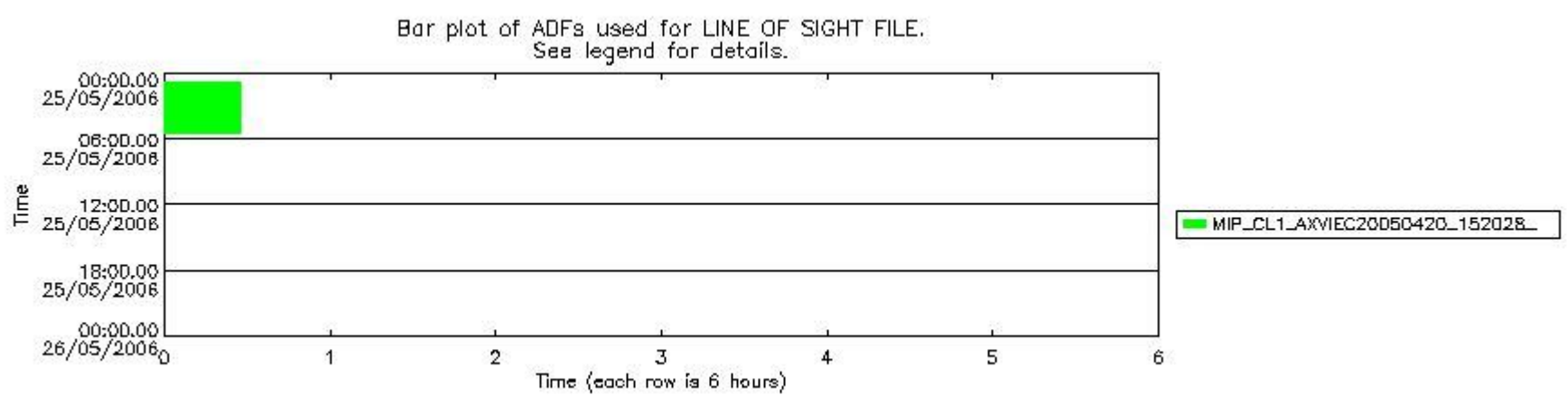
mipas_daily_report_level1_OFI_MIPAS_4_65_P_20060525_53.PNG
