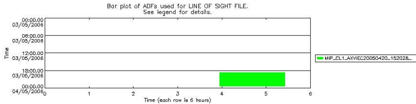
mipas_daily_report_level1_OFI_MIPAS_4_65_P_20060503_53.PNG
