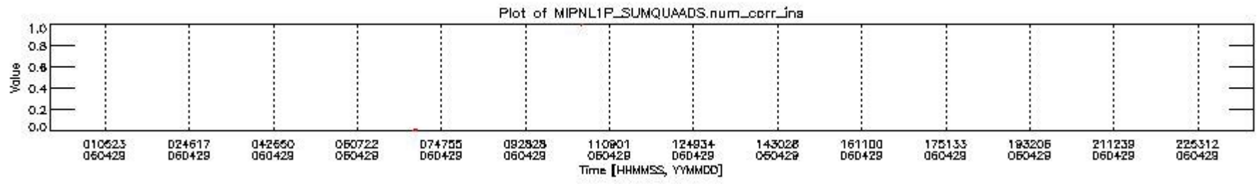
mipas_daily_report_level1_OFI_MIPAS_4_65_P_20060429_4.PNG
