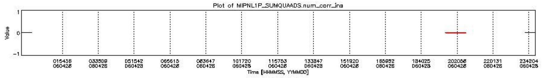
mipas_daily_report_level1_OFI_MIPAS_4_65_P_20060428_4.PNG
