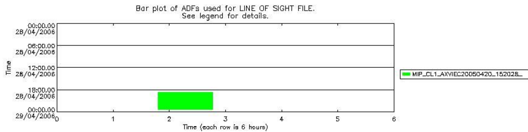
mipas_daily_report_level1_OFI_MIPAS_4_65_P_20060428_53.PNG
