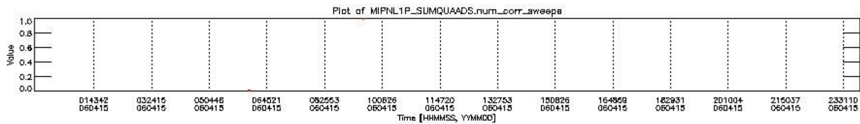
mipas_daily_report_level1_OFI_MIPAS_4_65_P_20060415_2.PNG
