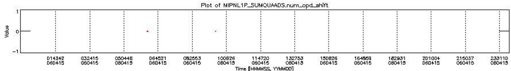
mipas_daily_report_level1_OFL_MIPAS_4_65_P_20060415_10.PNG
