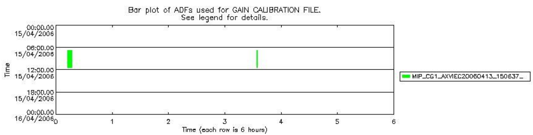
mipas_daily_report_level1_OFL_MIPAS_4_65_P_20060415_52.PNG
