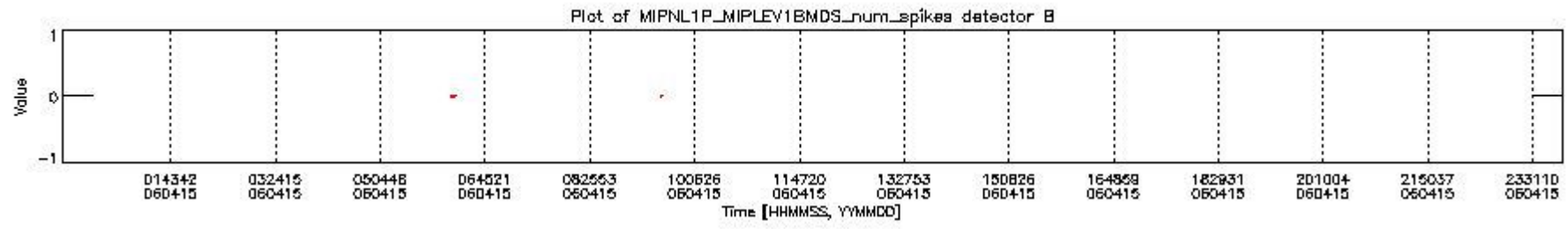
mipas_daily_report_level1_OFL_MIPAS_4_65_P_20060415_22.PNG
