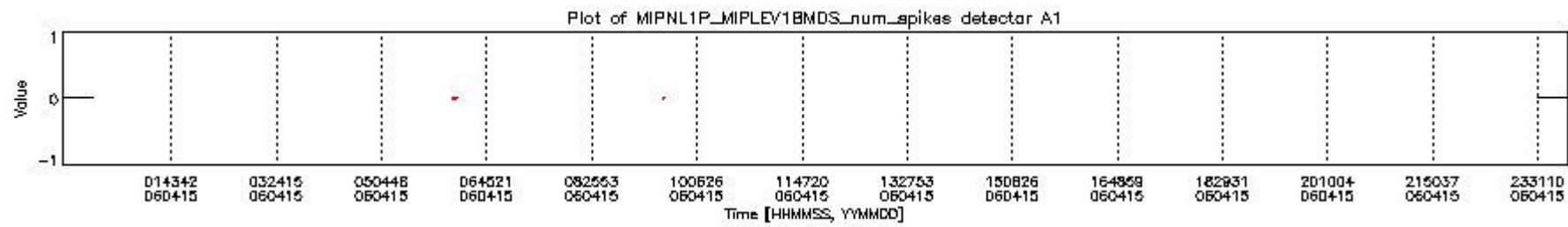
mipas_daily_report_level1_OFL_MIPAS_4_65_P_20060415_16.PNG
