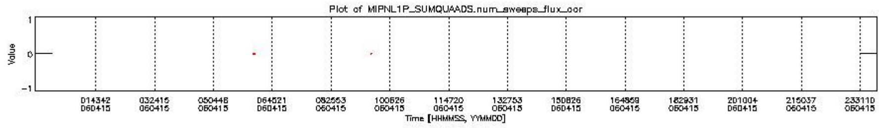
mipas_daily_report_level1_OFL_MIPAS_4_65_P_20060415_12.PNG
