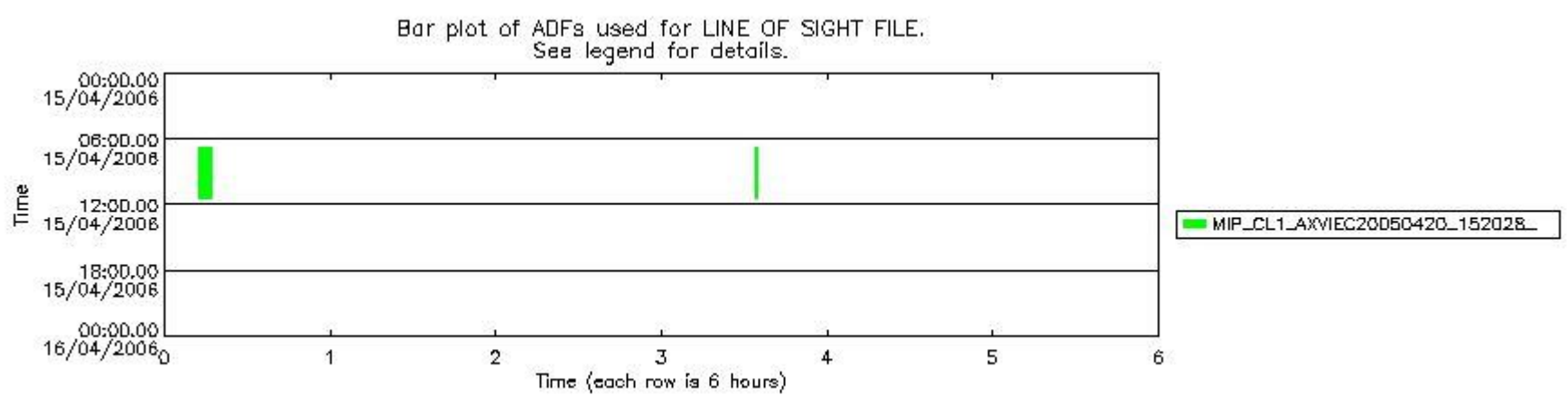
mipas_daily_report_level1_OFL_MIPAS_4_65_P_20060415_53.PNG
