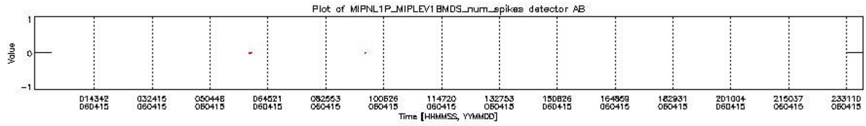
mipas_daily_report_level1_OFL_MIPAS_4_65_P_20060415_20.PNG
