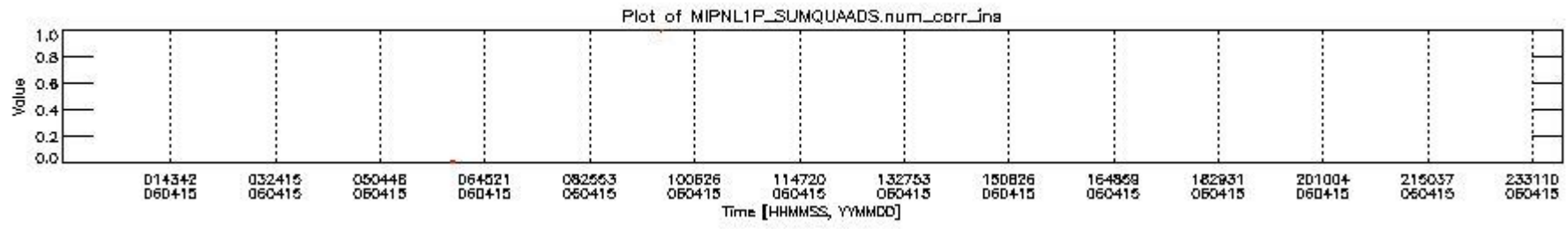
mipas_daily_report_level1_OFI_MIPAS_4_65_P_20060415_4.PNG
