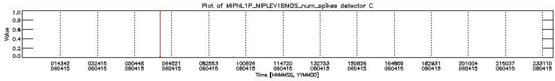
mipas_daily_report_level1_OFI_MIPAS_4_65_P_20060415_24.PNG
