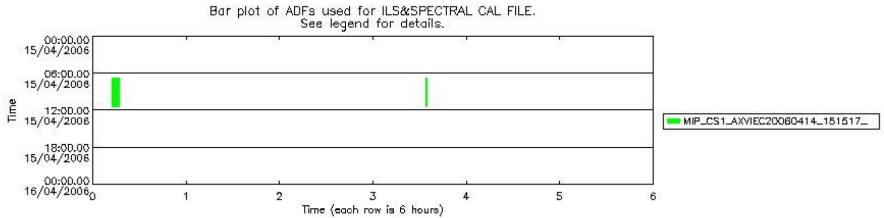
mipas_daily_report_level1_OFL_MIPAS_4_65_P_20060415_51.PNG
