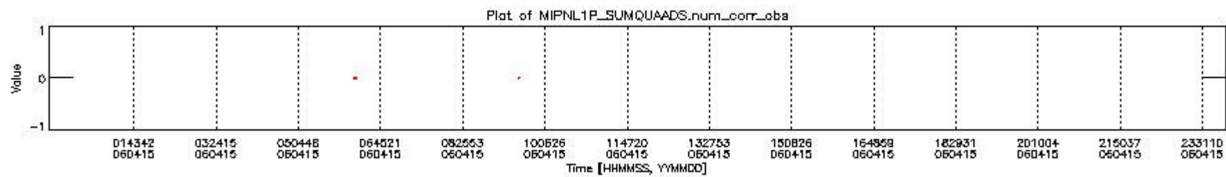
mipas_daily_report_level1_OFI_MIPAS_4_65_P_20060415_6.PNG
