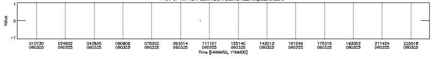
mipas_daily_report_level1_OFI_MIPAS_4_65_P_20060325_12.PNG
