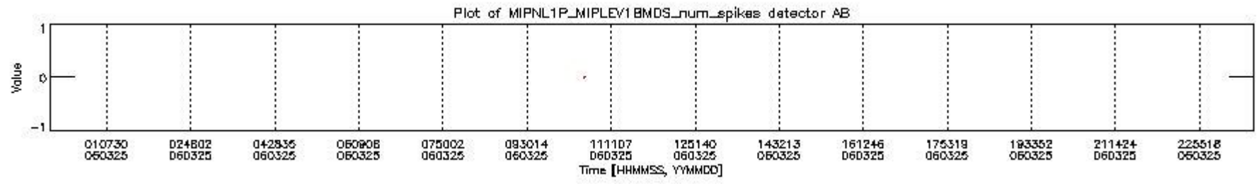
mipas_daily_report_level1_OFI_MIPAS_4_65_P_20060325_20.PNG
