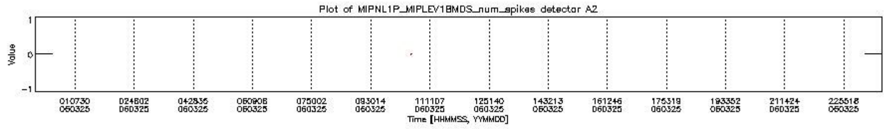
mipas_daily_report_level1_OFI_MIPAS_4_65_P_20060325_18.PNG
