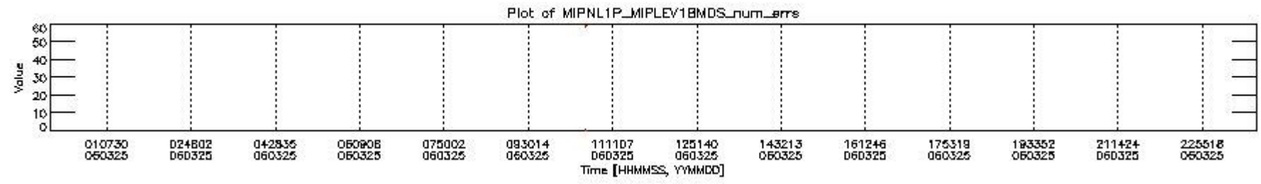
mipas_daily_report_level1_OFI_MIPAS_4_65_P_20060325_28.PNG
