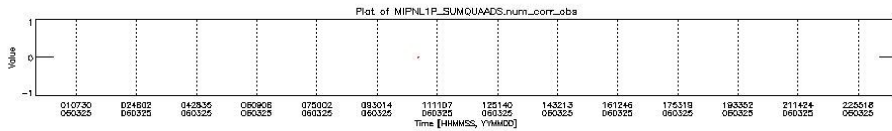
mipas_daily_report_level1_OFI_MIPAS_4_65_P_20060325_6.PNG
