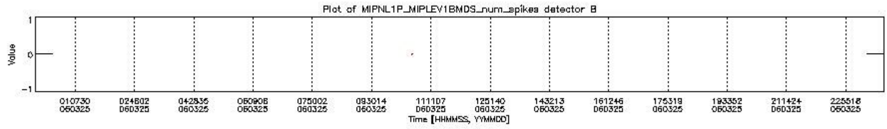
mipas_daily_report_level1_OFI_MIPAS_4_65_P_20060325_22.PNG
