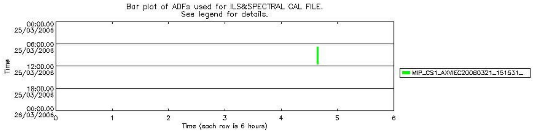
mipas_daily_report_level1_OFI_MIPAS_4_65_P_20060325_51.PNG
