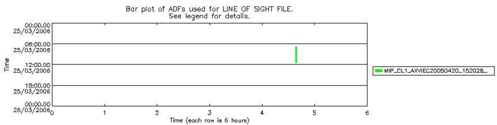
mipas_daily_report_level1_OFI_MIPAS_4_65_P_20060325_53.PNG
