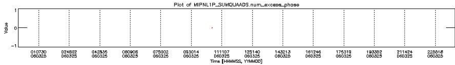
mipas_daily_report_level1_OFI_MIPAS_4_65_P_20060325_8.PNG
