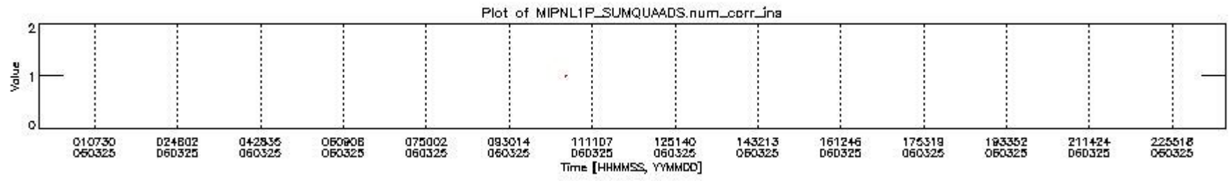
mipas_daily_report_level1_OFI_MIPAS_4_65_P_20060325_4.PNG
