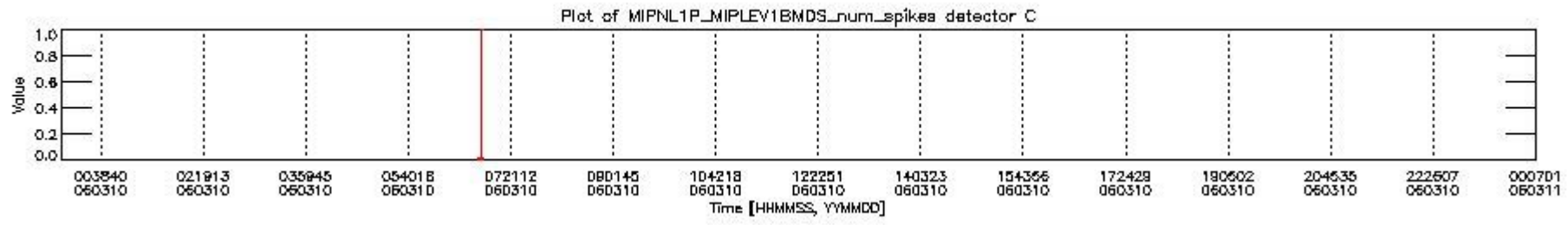
mipas_daily_report_level1_OFI_MIPAS_4_65_P_20060310_24.PNG
