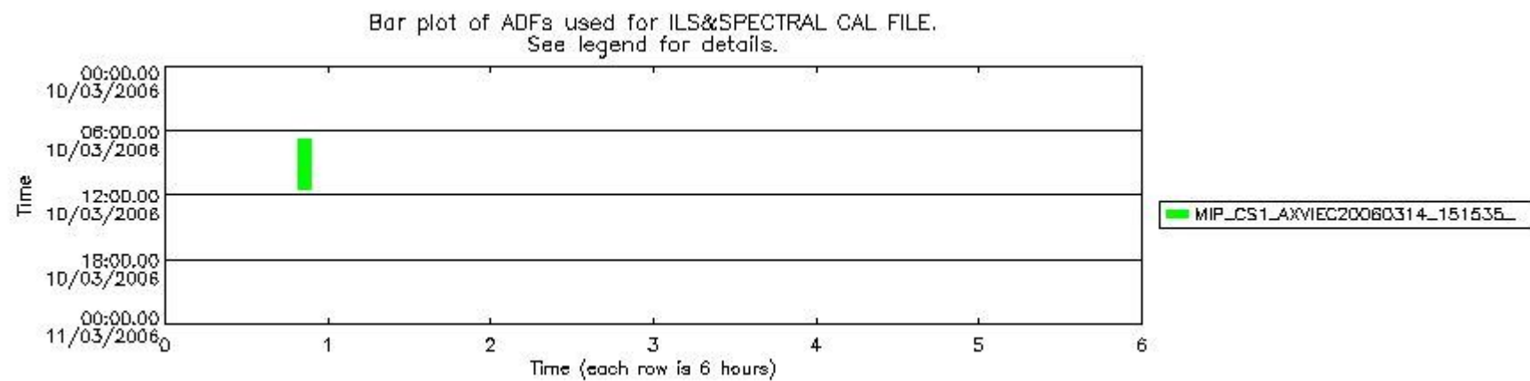
mipas_daily_report_level1_OFI_MIPAS_4_65_P_20060310_51.PNG
