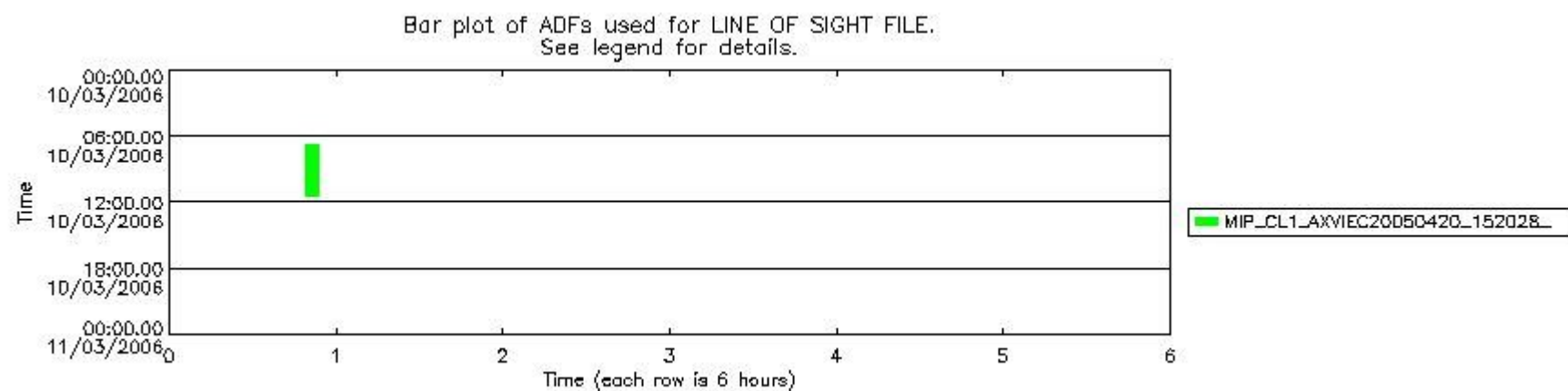
mipas_daily_report_level1_OFI_MIPAS_4_65_P_20060310_53.PNG
