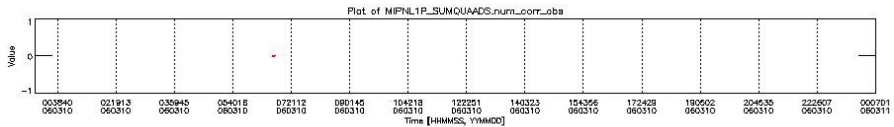
mipas_daily_report_level1_OFI_MIPAS_4_65_P_20060310_6.PNG
