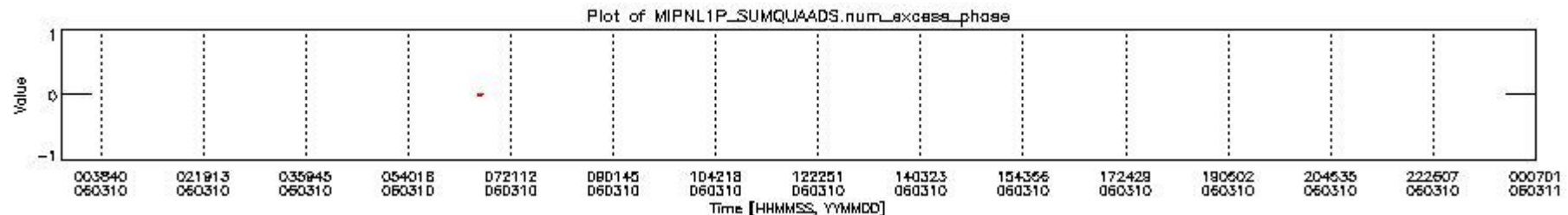
mipas_daily_report_level1_OFI_MIPAS_4_65_P_20060310_8.PNG
