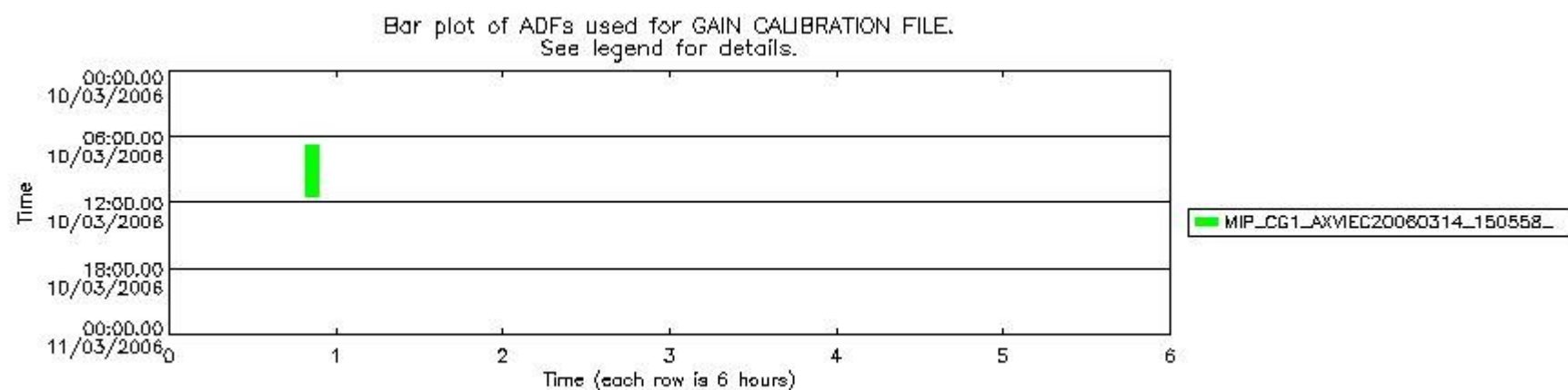
mipas_daily_report_level1_OFI_MIPAS_4_65_P_20060310_52.PNG
