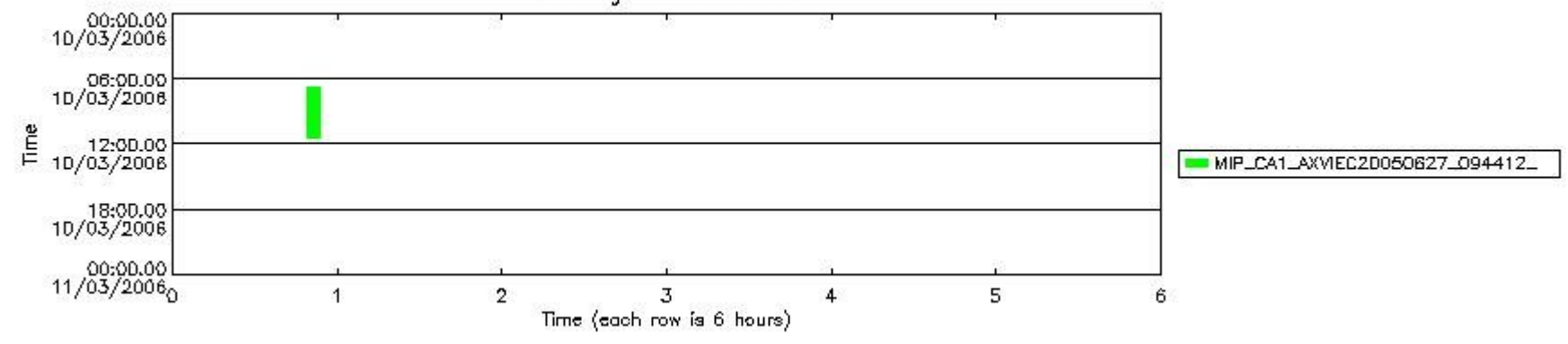
mipas_daily_report_level1_OFL_MIPAS_4_65_P_20060310_54.PNG
