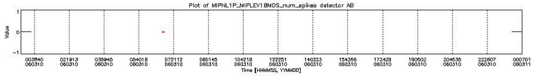
mipas_daily_report_level1_OFI_MIPAS_4_65_P_20060310_20.PNG
