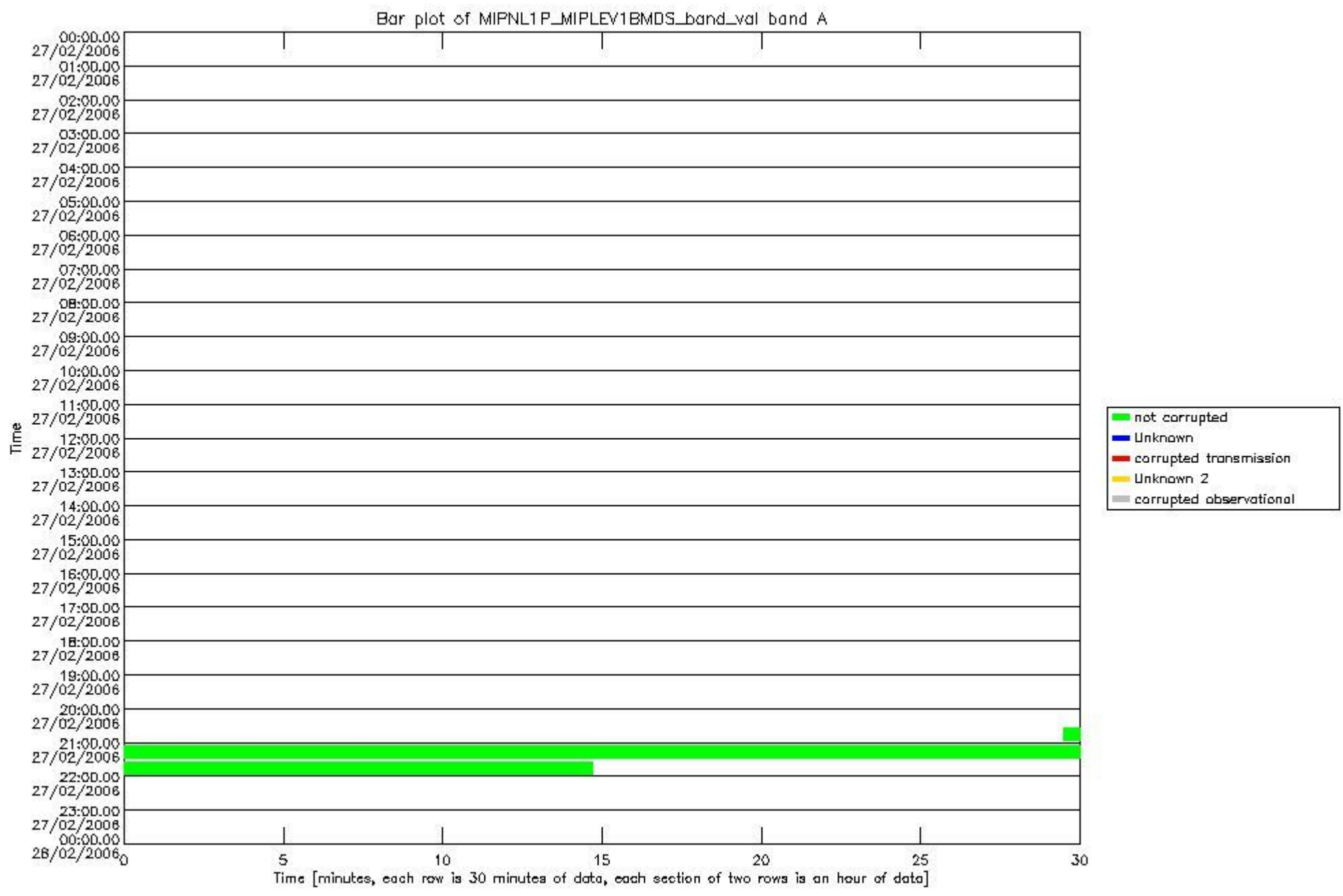
mipas_daily_report_level1_OFI_MIPAS_4_65_P_20060227_30.PNG
