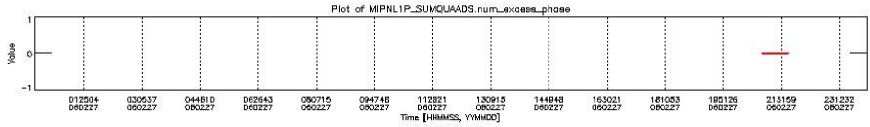
mipas_daily_report_level1_OFI_MIPAS_4_65_P_20060227_8.PNG
