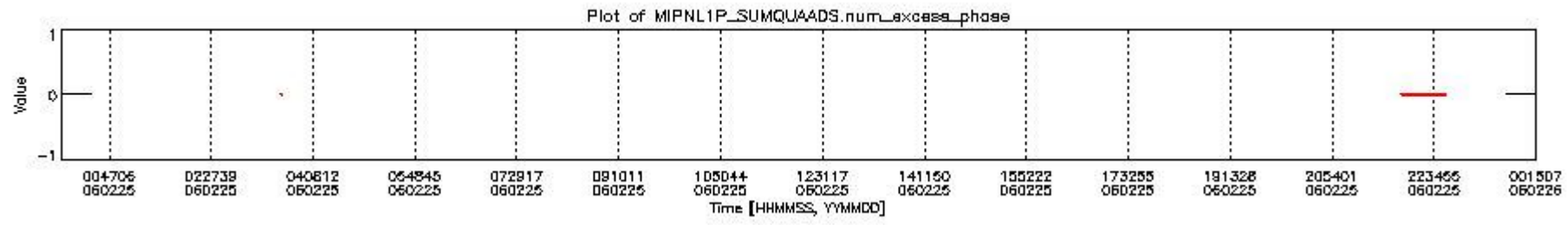
mipas_daily_report_level1_OFI_MIPAS_4_65_P_20060225_8.PNG
