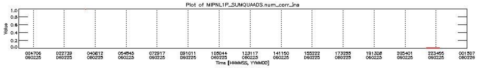
mipas_daily_report_level1_OFI_MIPAS_4_65_P_20060225_4.PNG
