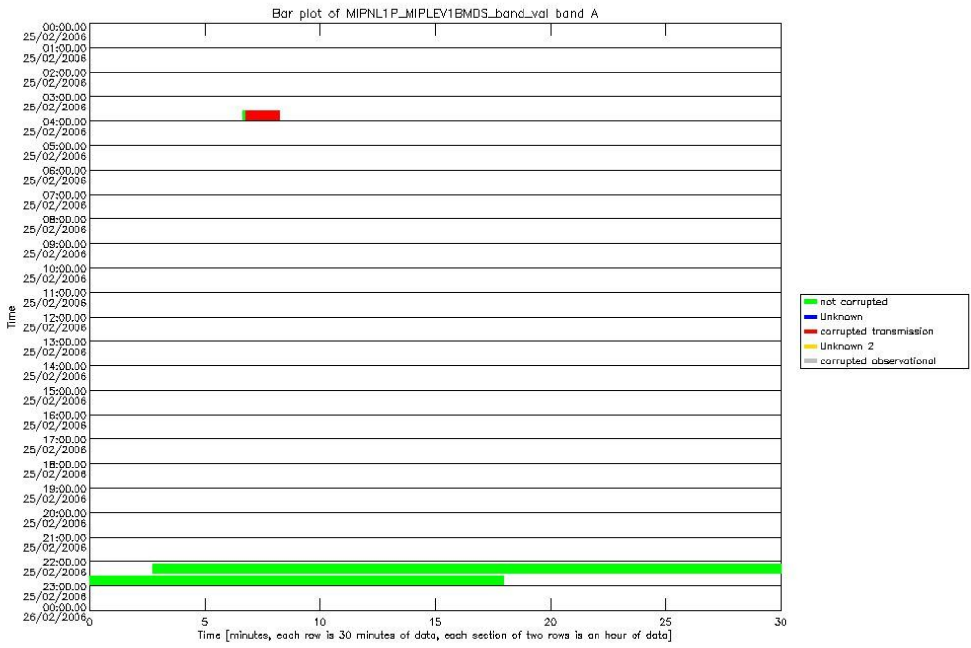
mipas_daily_report_level1_OFI_MIPAS_4_65_P_20060225_30.PNG
