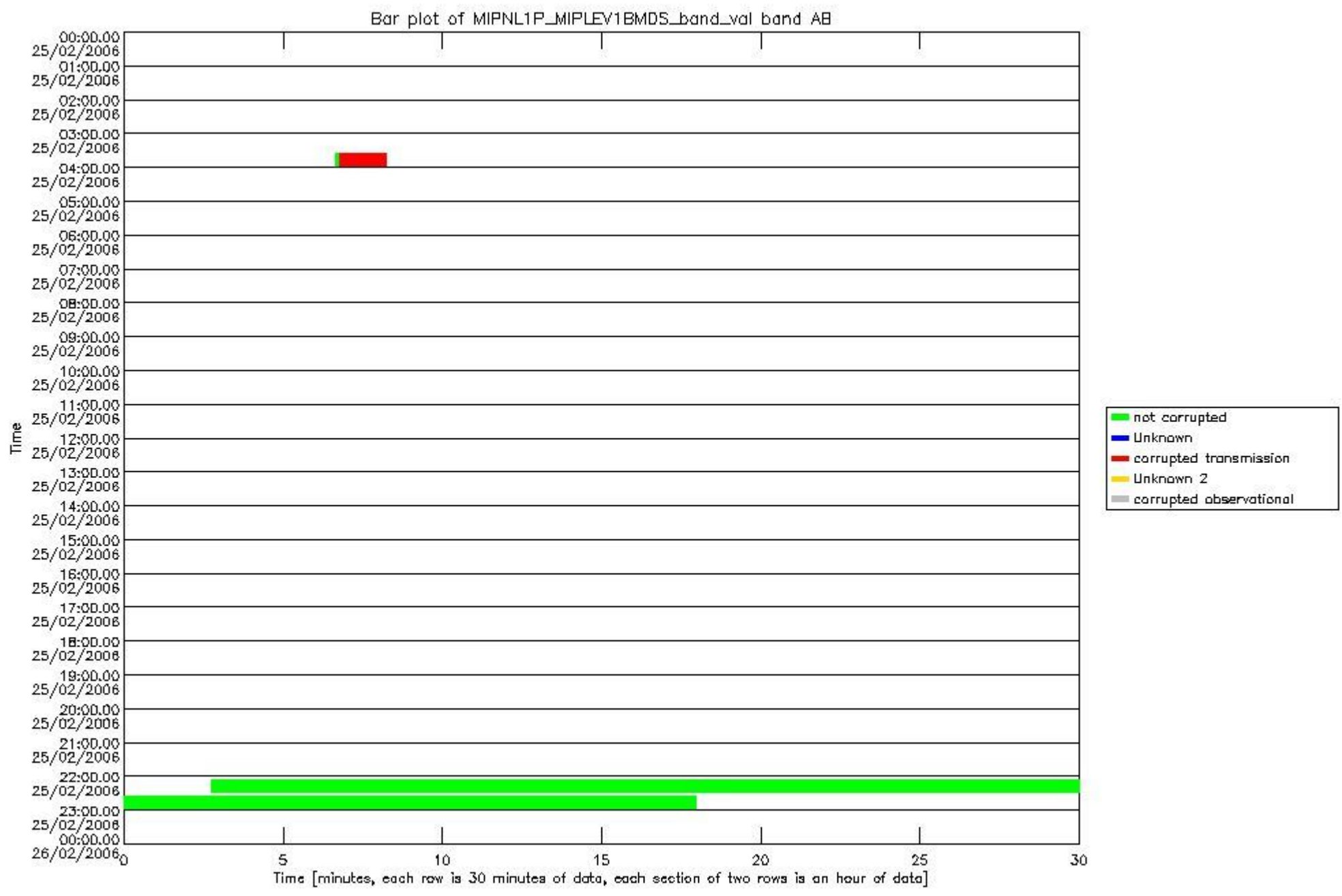
mipas_daily_report_level1_OFI_MIPAS_4_65_P_20060225_32.PNG
