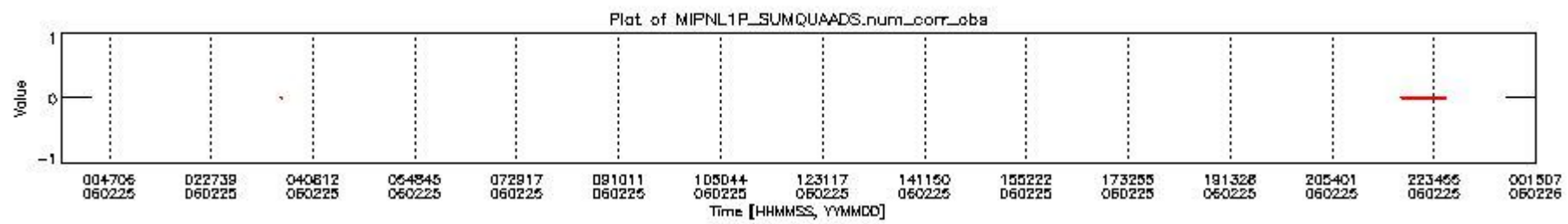
mipas_daily_report_level1_OFI_MIPAS_4_65_P_20060225_6.PNG
