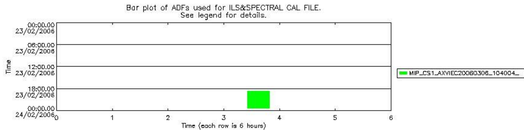
mipas_daily_report_level1_OFI_MIPAS_4_65_P_20060223_51.PNG
