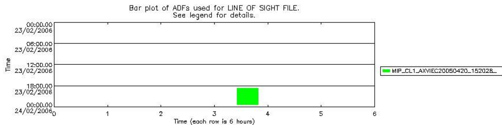
mipas_daily_report_level1_OFI_MIPAS_4_65_P_20060223_53.PNG
