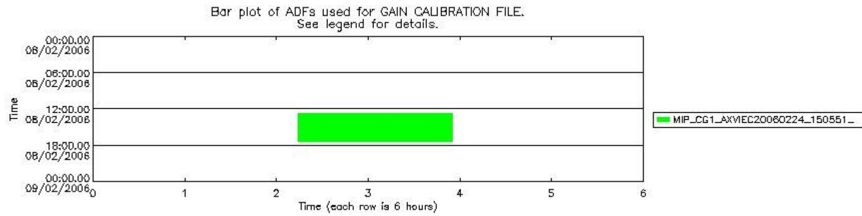
mipas_daily_report_level1_OFI_MIPAS_4_65_P_20060208_53.PNG
