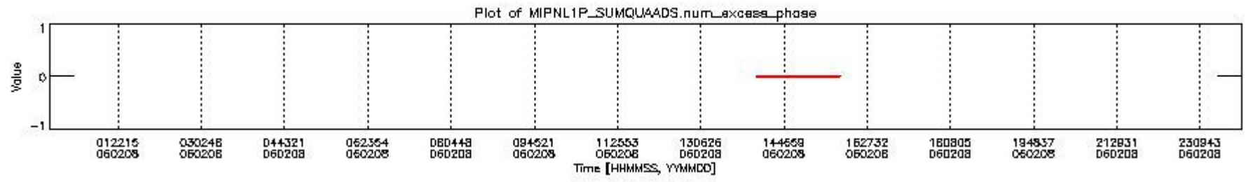
mipas_daily_report_level1_OFI_MIPAS_4_65_P_20060208_8.PNG
