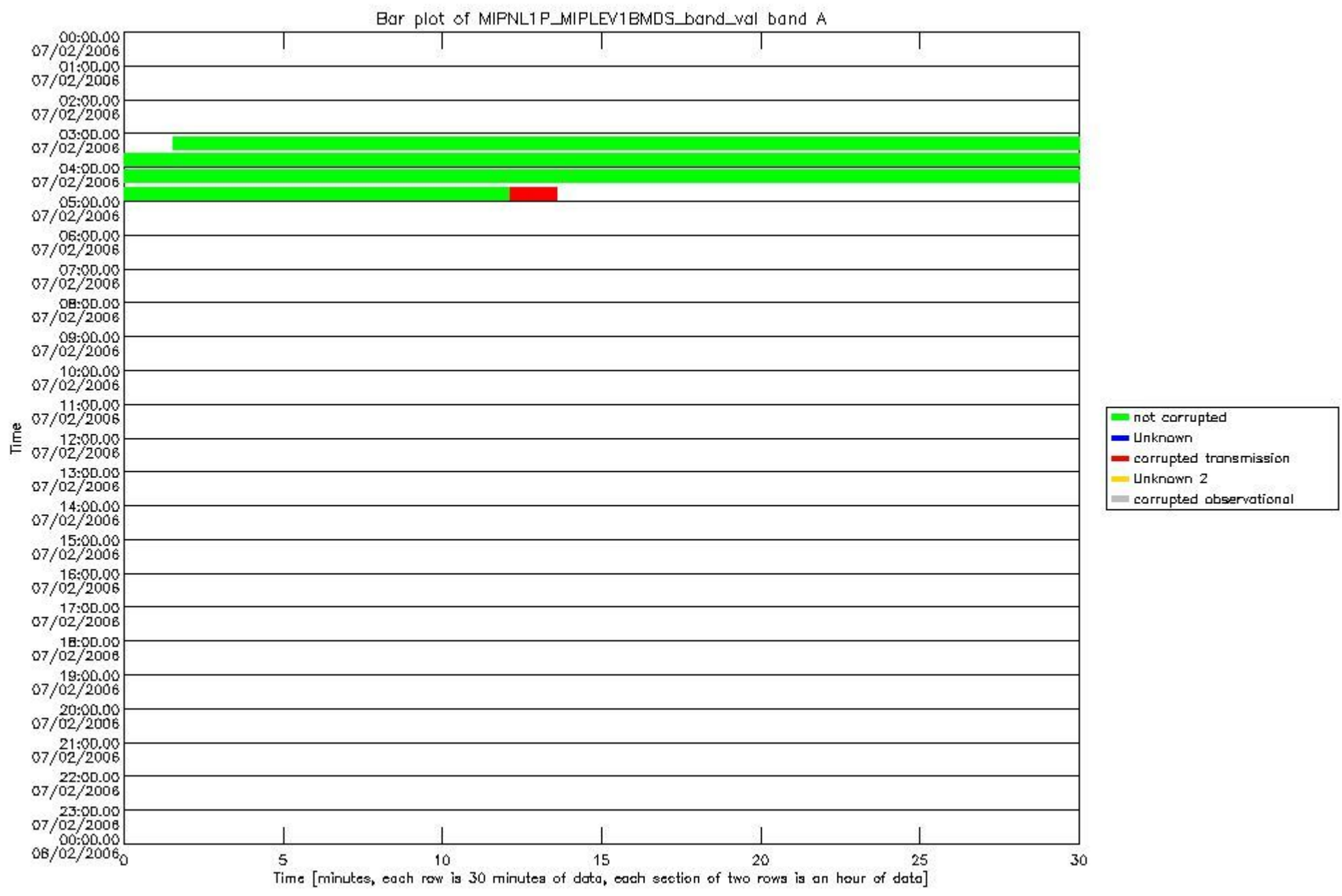
mipas_daily_report_level1_OFI_MIPAS_4_65_P_20060207_30.PNG
