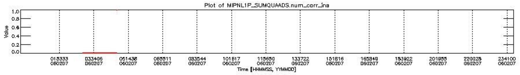
mipas_daily_report_level1_OFI_MIPAS_4_65_P_20060207_4.PNG
