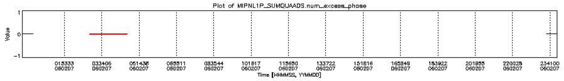
mipas_daily_report_level1_OFI_MIPAS_4_65_P_20060207_8.PNG
