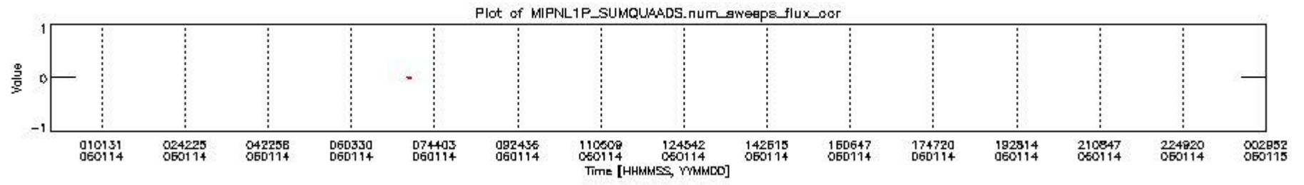
mipas_daily_report_level1_OFI_MIPAS_4_65_P_20060114_12.PNG
