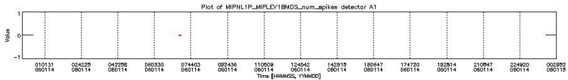
mipas_daily_report_level1_OFL_MIPAS_4_65_P_20060114_16.PNG
