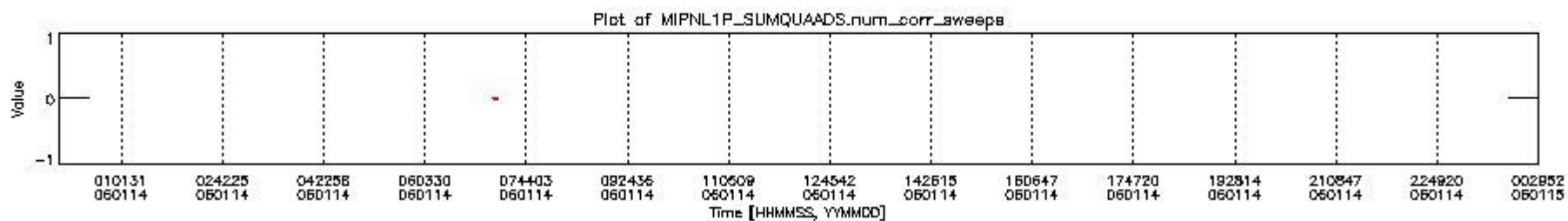
mipas_daily_report_level1_OFI_MIPAS_4_65_P_20060114_2.PNG
