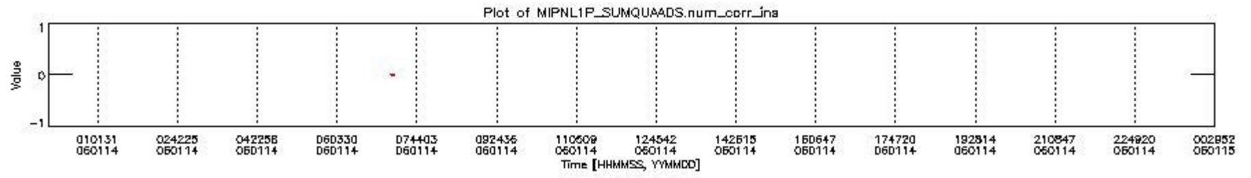
mipas_daily_report_level1_OFI_MIPAS_4_65_P_20060114_4.PNG
