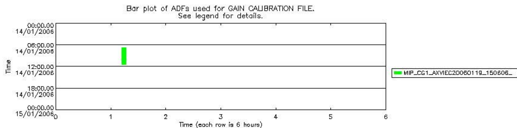
mipas_daily_report_level1_OFI_MIPAS_4_65_P_20060114_52.PNG
