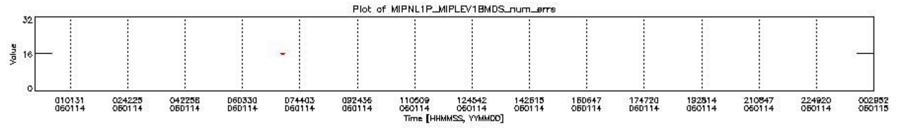
mipas_daily_report_level1_OFI_MIPAS_4_65_P_20060114_28.PNG
