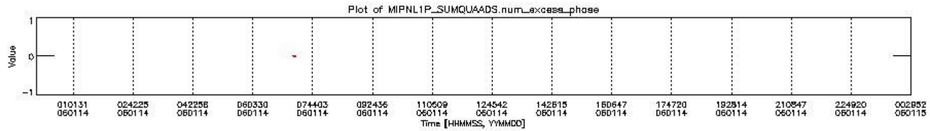
mipas_daily_report_level1_OFI_MIPAS_4_65_P_20060114_8.PNG
