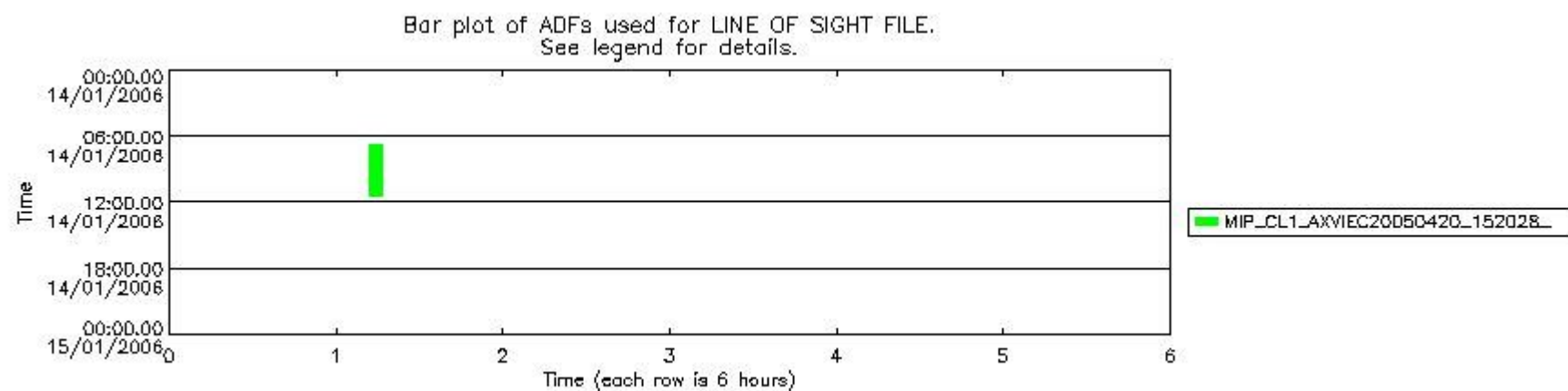
mipas_daily_report_level1_OFI_MIPAS_4_65_P_20060114_53.PNG
