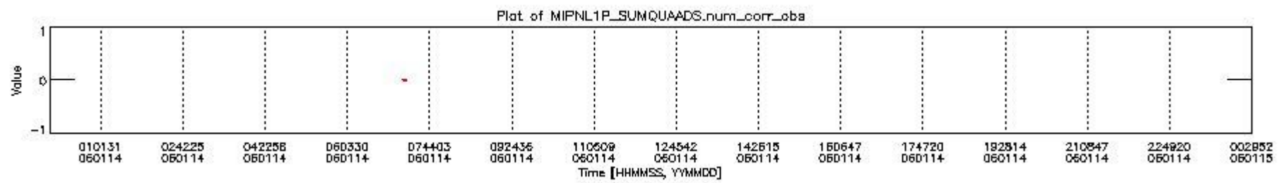
mipas_daily_report_level1_OFI_MIPAS_4_65_P_20060114_6.PNG
