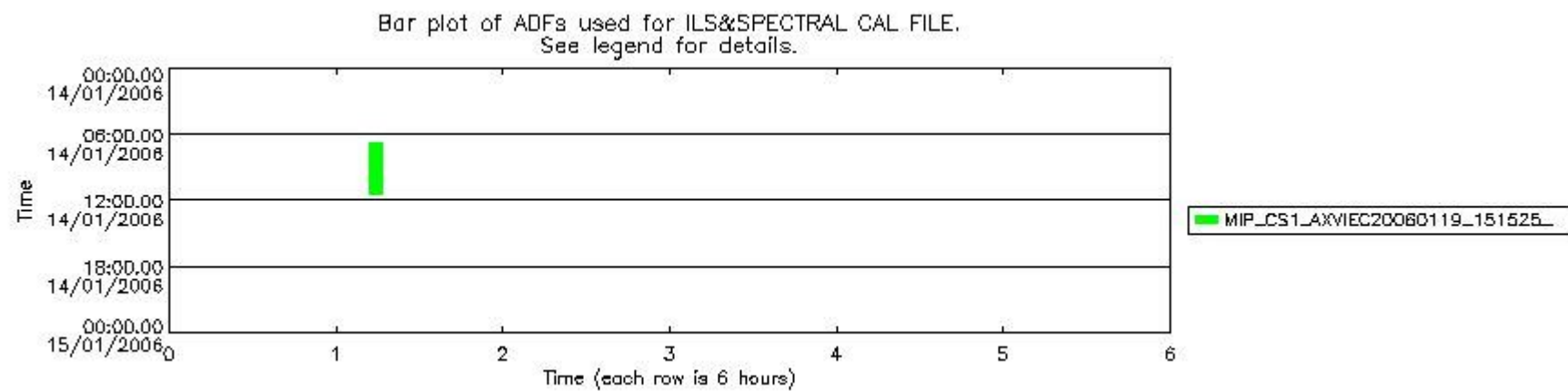
mipas_daily_report_level1_OFI_MIPAS_4_65_P_20060114_51.PNG
