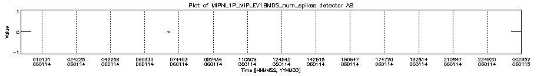
mipas_daily_report_level1_OFI_MIPAS_4_65_P_20060114_20.PNG
