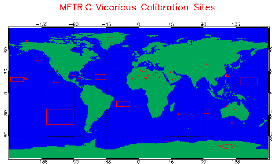
Figure 12 – Map of METRIC Calibration Sites
