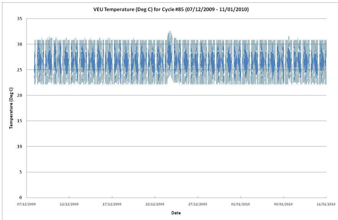
Figure 11 – VEU Temperature during Cycle #85
