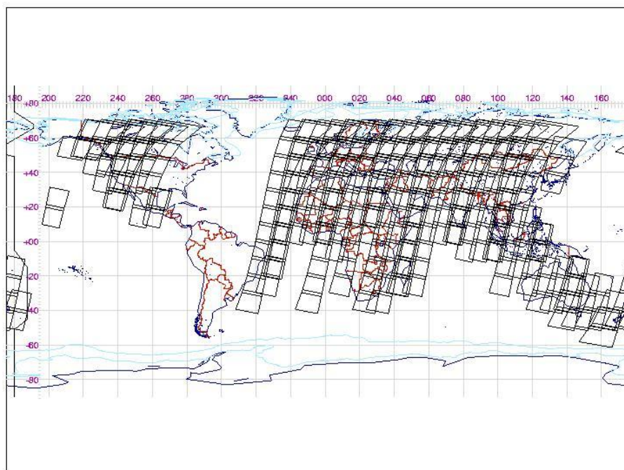
Figure 4 – MERIS FULL RESOLUTION LEVEL 0 ACQUISITIONS – PART #2 – 03/11/2009 – 07/11/2009
