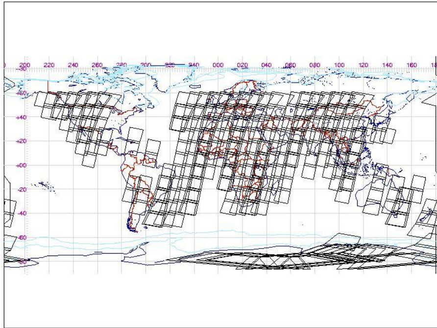
Figure 3 – MERIS FULL RESOLUTION LEVEL 0 ACQUISITIONS – PART #1 –22/01/2009 – 26/01/2009
