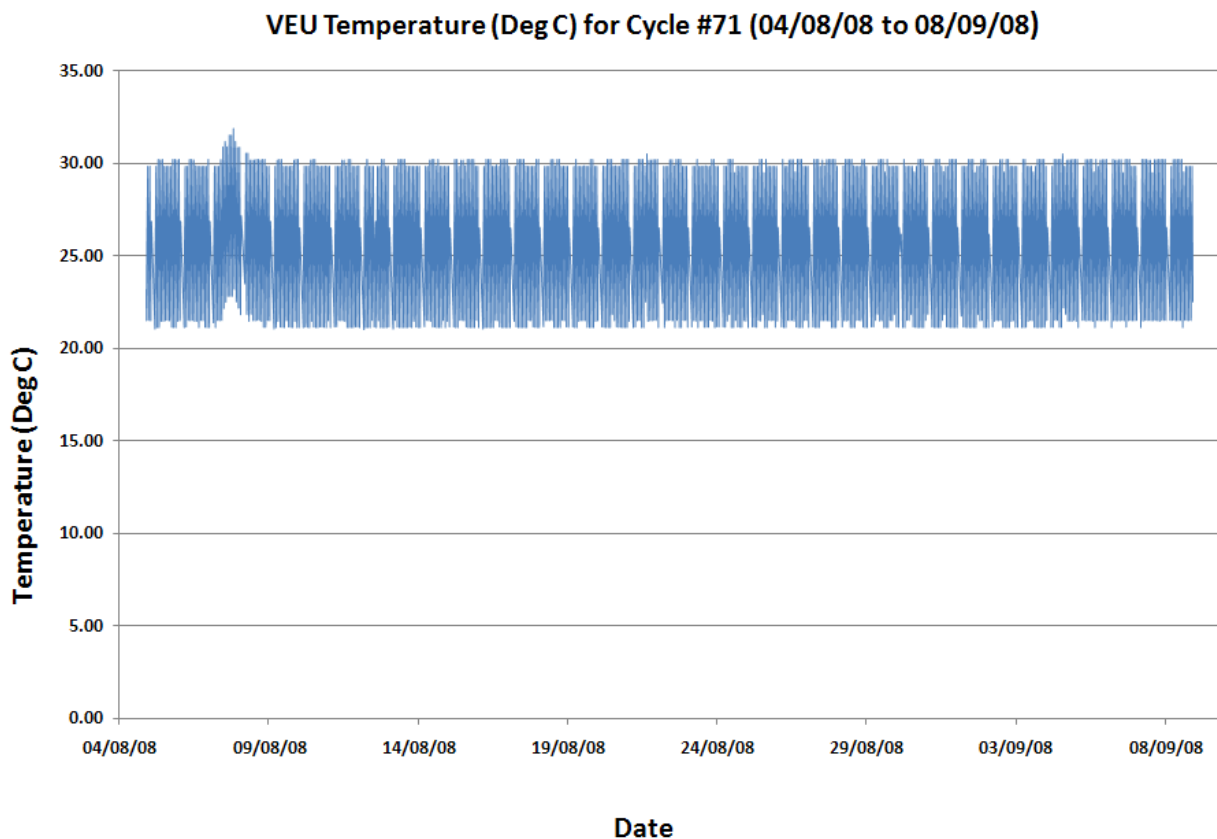
Figure 10 – VEU TEMPERATURE DURING CYCLE #71
