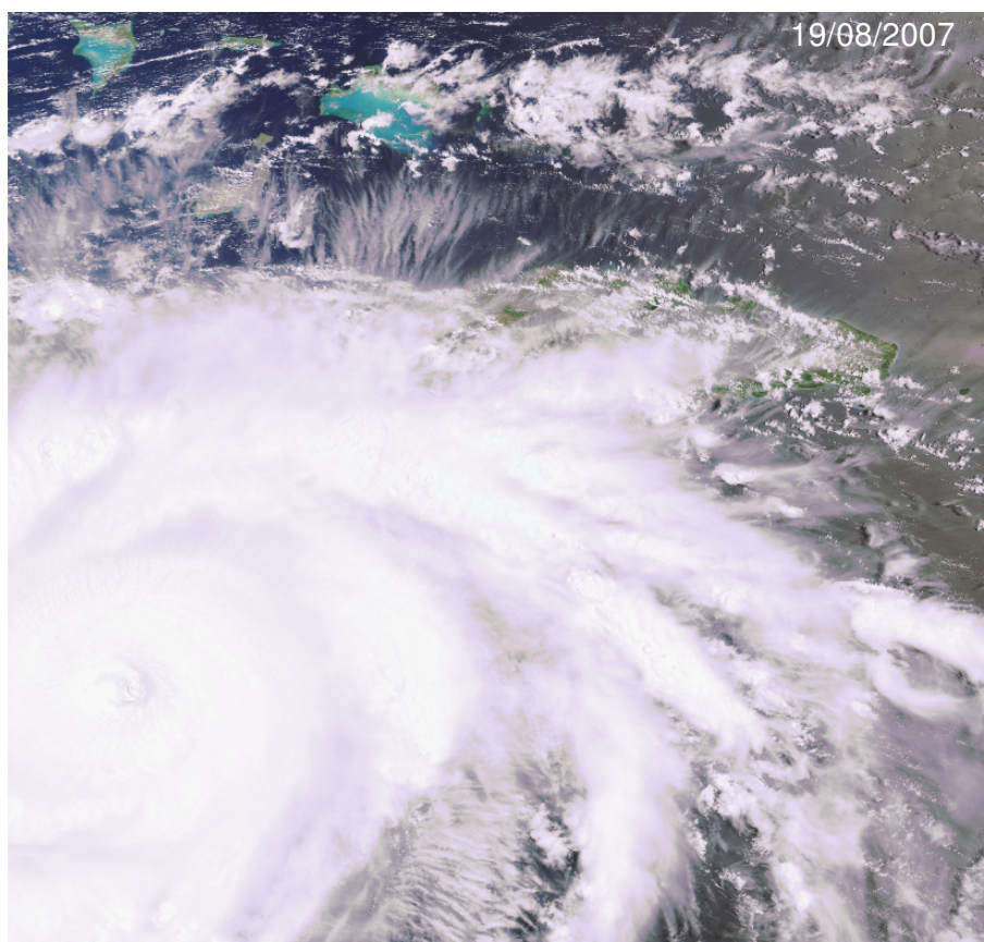
Hurricane Dean - MERIS reduced resolution scene - South-West of the Dominican Republic
