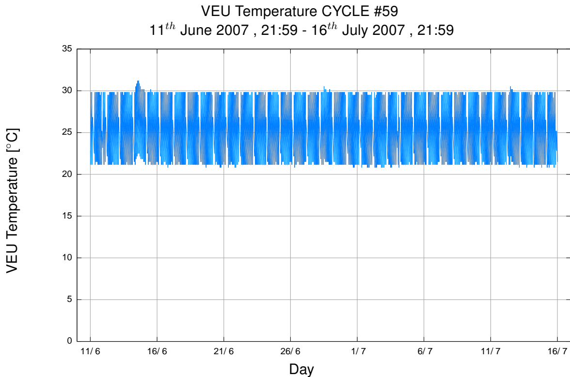
Figure 10: VEU Temperature during cycle #59
