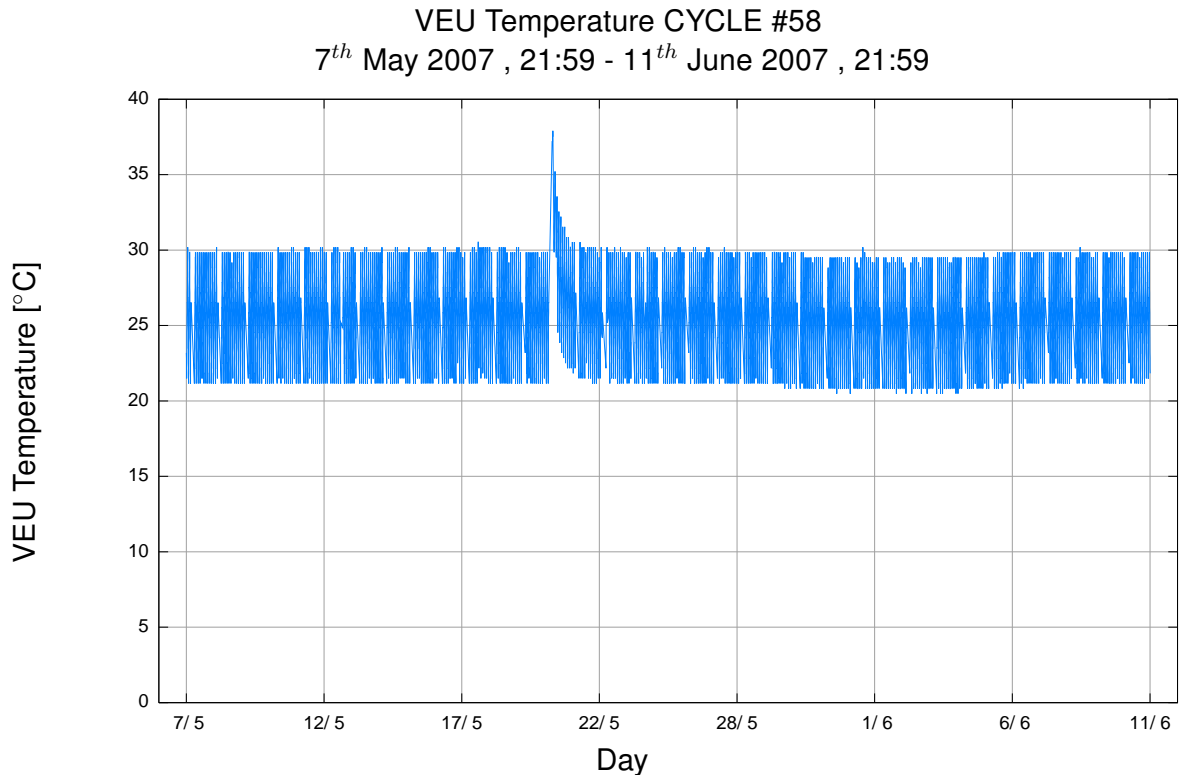
Figure 10: VEU Temperature during cycle #58
