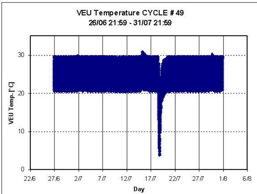
Figure 10 - VEU Temperature during cycle #49
