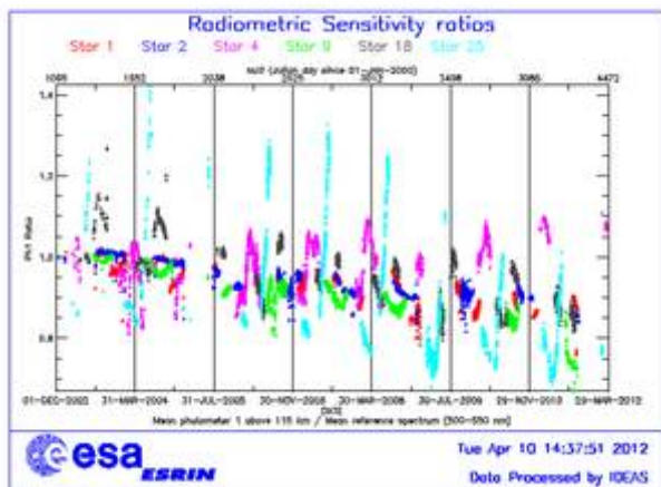
Figure 5.4-1: Radiometric sensitivity ratios since December 2002
