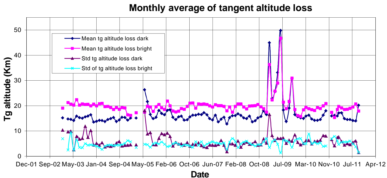
Figure 4.6-6: Monthly mean tangent altitude (and STD) at which the star is lost since January 2003
