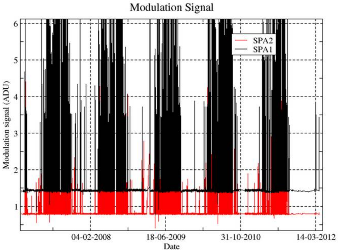
Figure 4.5-4: Modulation signal
