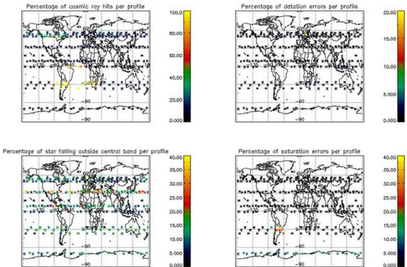
Figure 5.2-6: Level 1b product quality monitoring with respect to time DESCENDING ENVISAT passes
