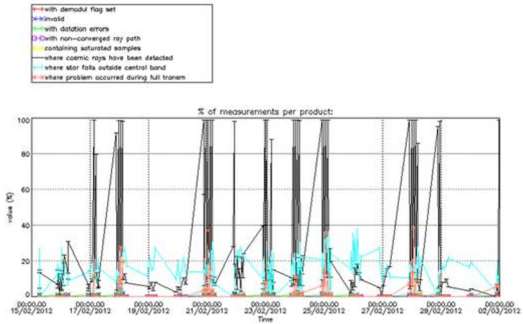
Figure 0-1: Level 1b product quality monitoring with respect to time
