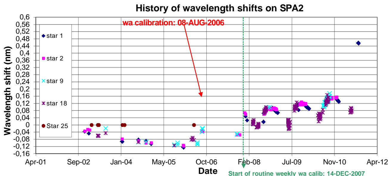
Figure 5.3-0-1: SPA2 wavelength monitoring since 12 th November 2002: for every star ID (1, 2, 9, 18, 25) it is plotted the spectral shift for which a maximum correlation has been found between the reference spectrum and the one of the occultation
