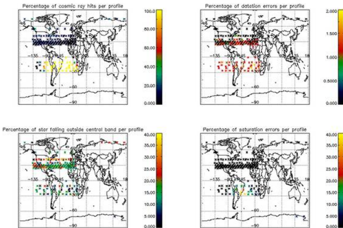
Figure 0-2: Level 1b product quality monitoring with respect to geolocation of ENVISAT
