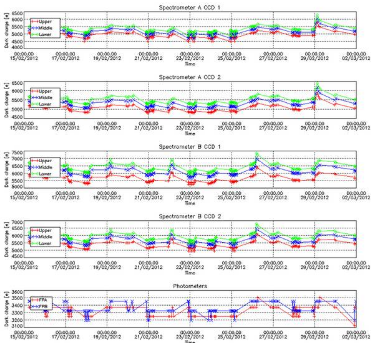
Figure 0-3: Mean Dark Charge of spectrometers and photometers during the reporting period
