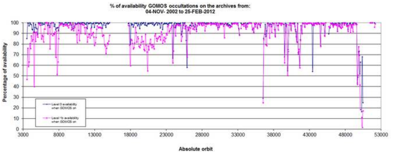
Figure 3.4-1: Percentage of level 0 and level 1b data availability on the archives PDHS-E and PDHS-K
