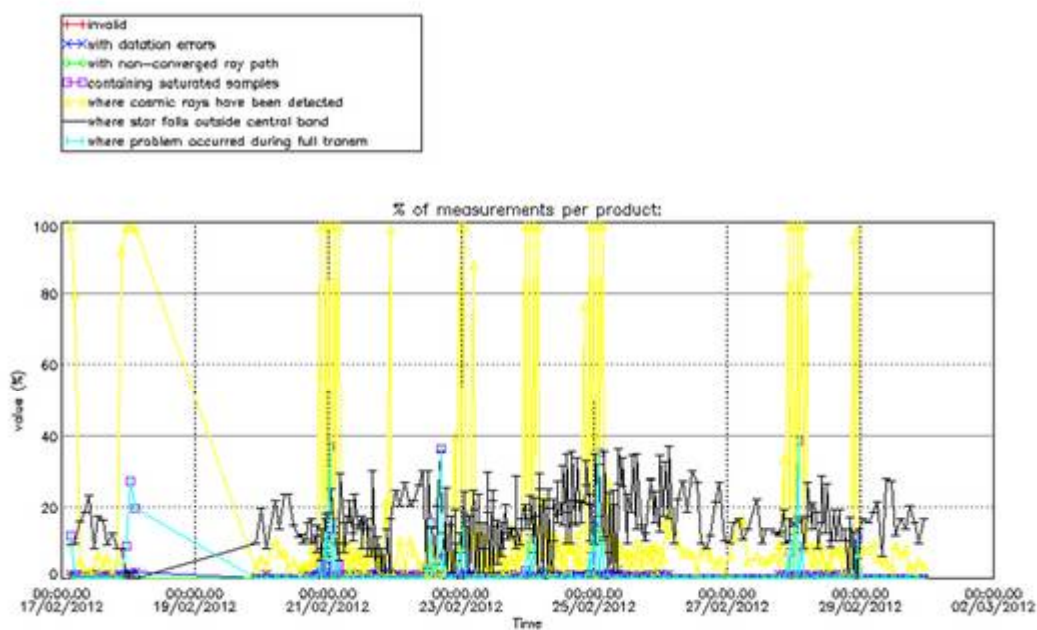
Figure 0-4: Level 1b product quality monitoring with respect to time ASCENDING ENVISAT passes
