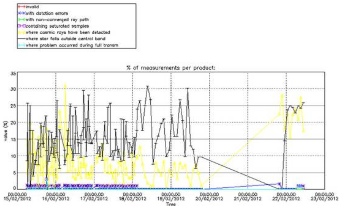
Figure 0-5: Level 1b product quality monitoring with respect to time DESCENDING ENVISAT passes
