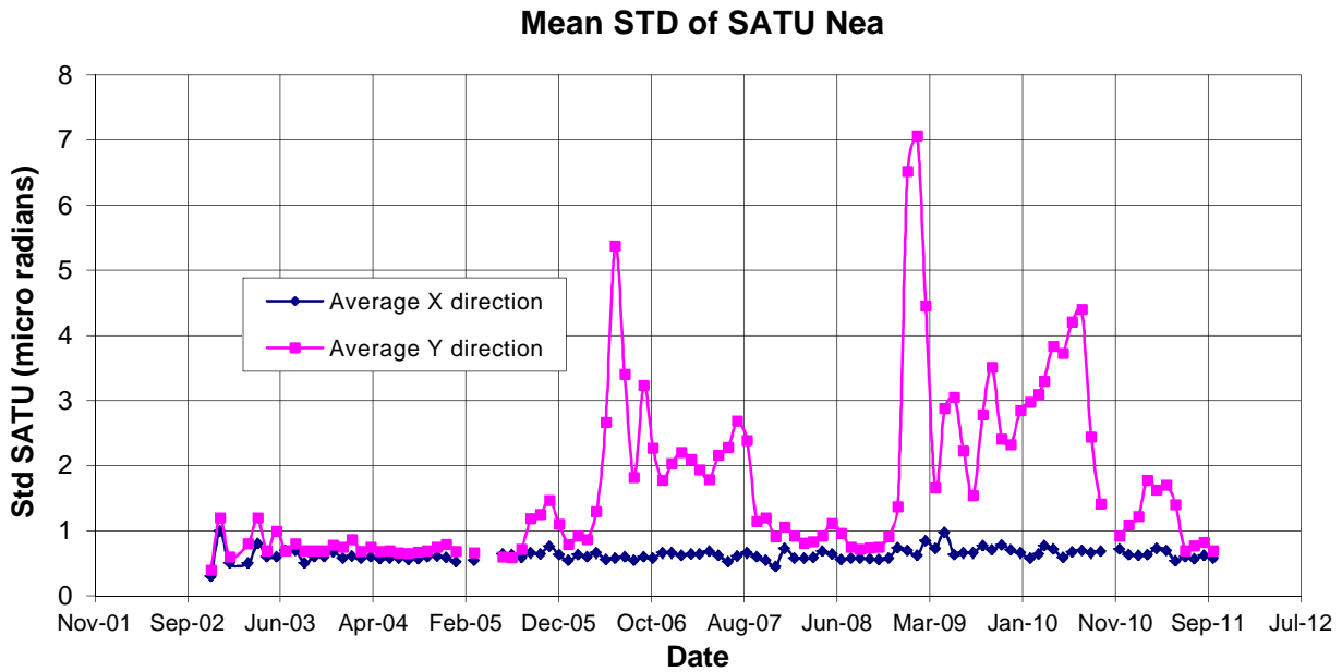
Figure 4.6-0-2: Average value per month of SATU NEA STD above 105 km
