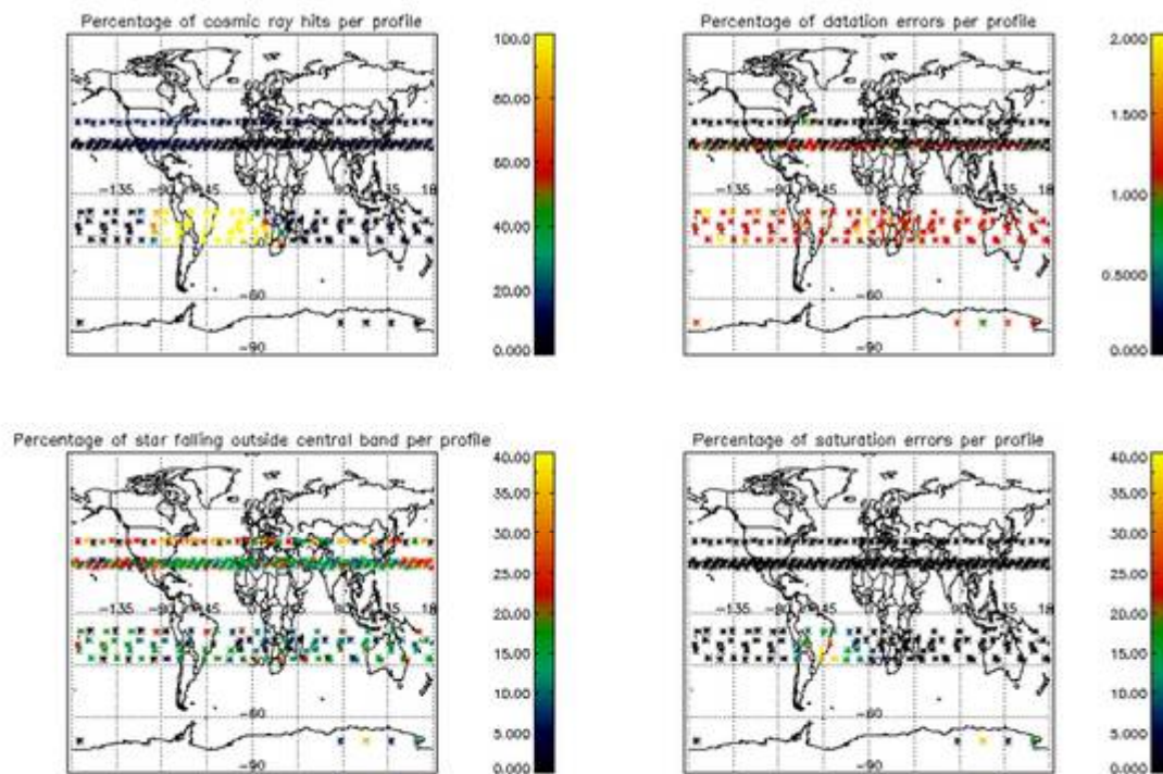
Figure 0-6: Level 1b product quality monitoring with respect to satellite geo-location for ASCENDING ENVISAT passes
