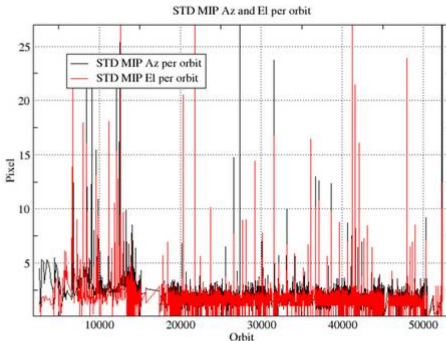
Figure 4.6-7: Standard deviation of MIP Azimuth and Elevation for some orbits since 1 st September 2002 until end of reporting period (see table 4.6-1)
