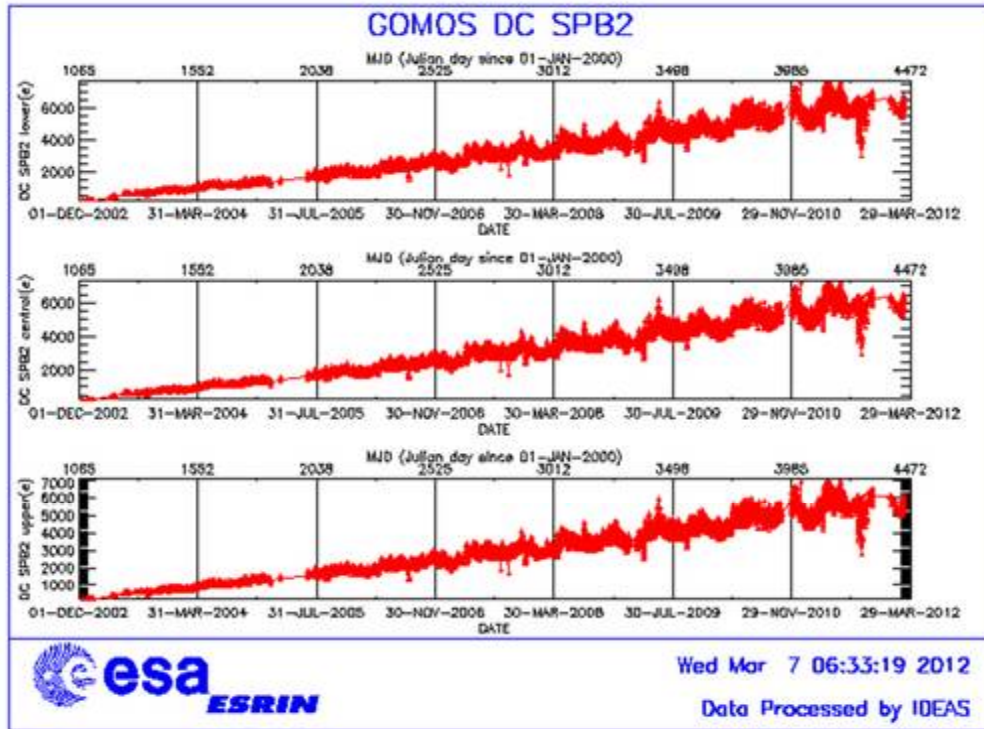
Figure 4.5-0-2: Mean DC evolution on SPB2 from 15 th December 2002
