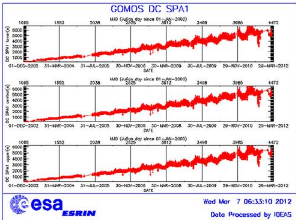
Figure 4.5-0-1: Mean DC evolution on SPA1 since 15 th December 2002
