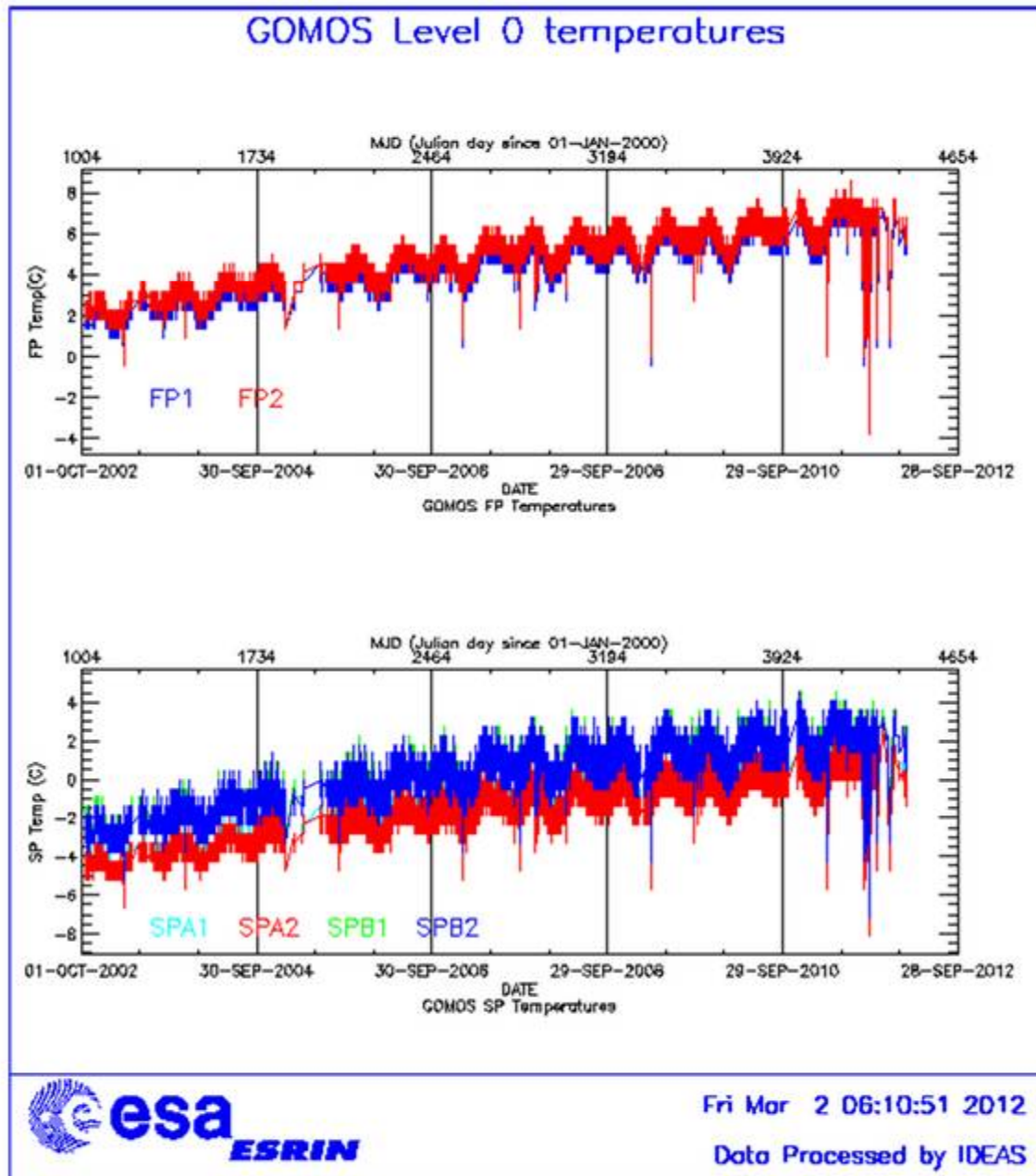
Figure 4.3-4.3-1: Level 0 temperature evolution of all GOMOS CCD detectors since October 2002
