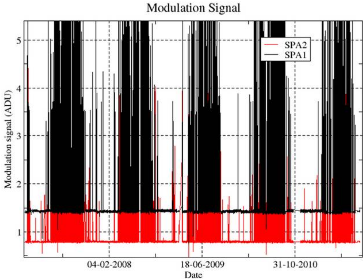
Figure 4.5-4: Modulation signal
