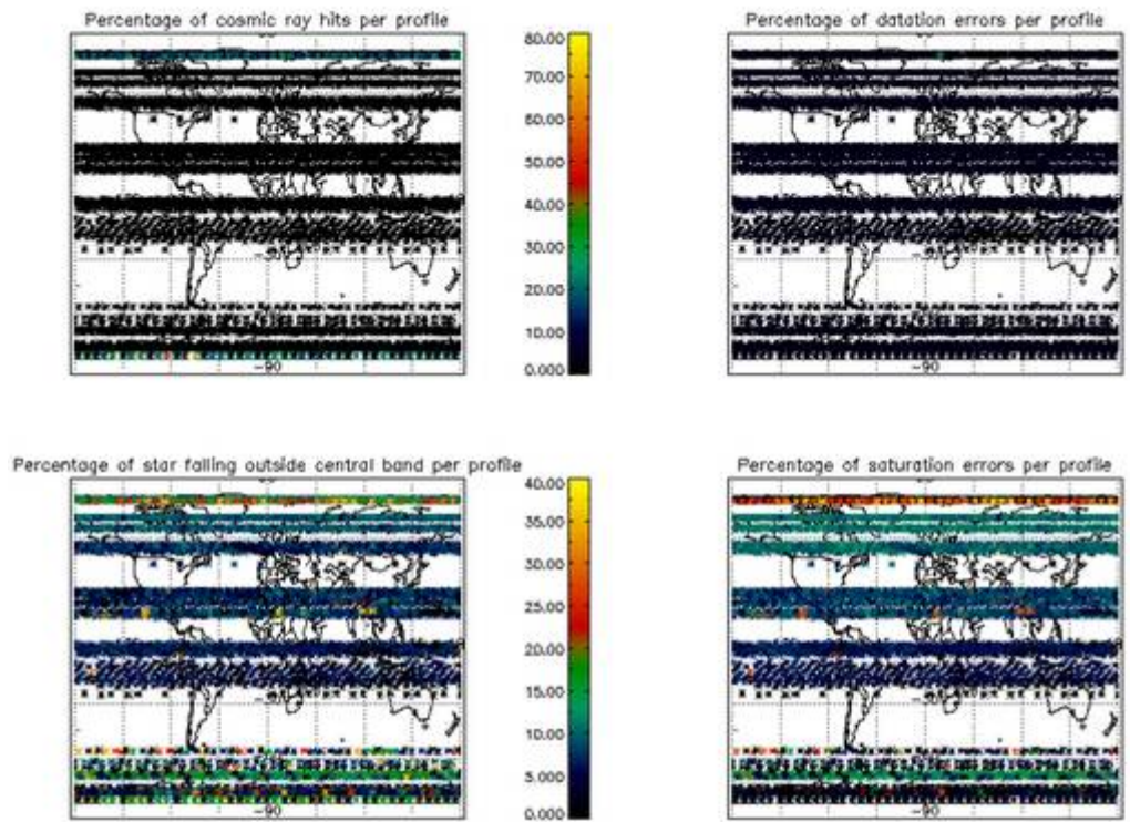
Figure 5.2-8: Level 1b product quality monitoring with respect to satellite geo-location for DESCENDING ENVISAT passes
