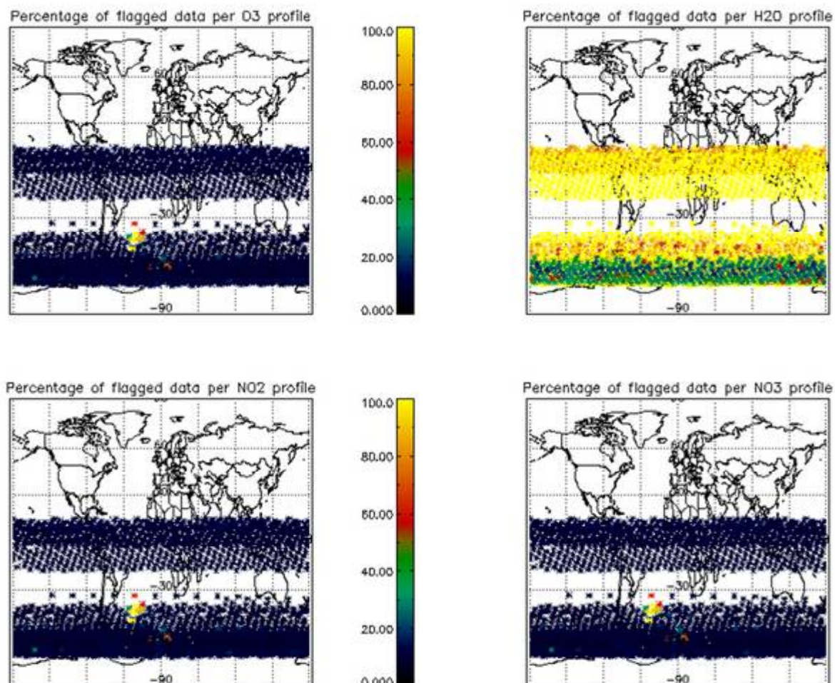
Figure 6.2-1: Percentage of flagged points per profile
