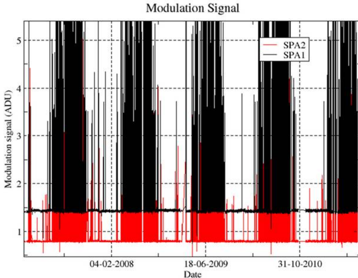
Figure 4.5-4: Modulation signal
