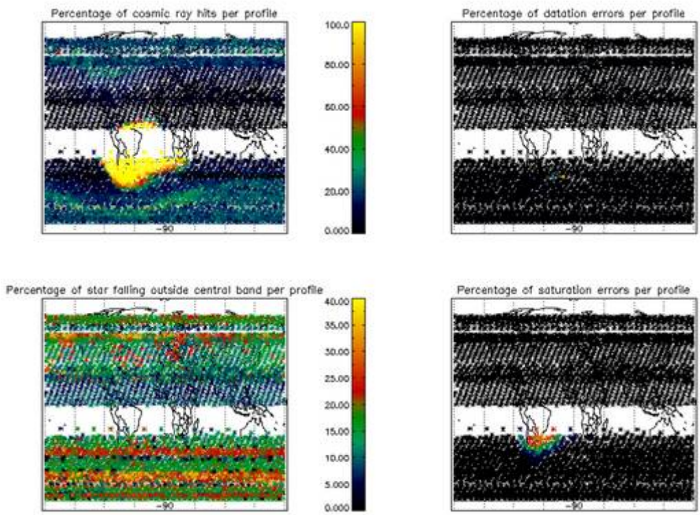
Figure 5.2-7: Level 1b product quality monitoring with respect to satellite geo-location for ASCENDING ENVISAT passes
