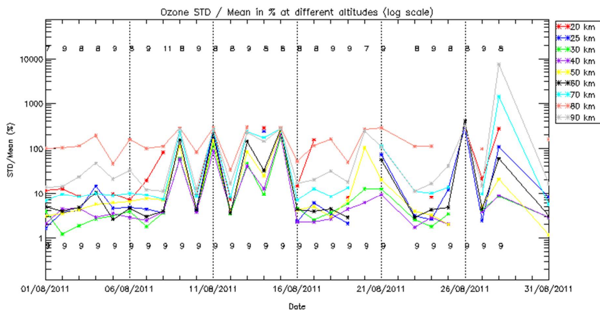
Figure 6.3-5: Daily dispersion defined as STD/Mean in %
