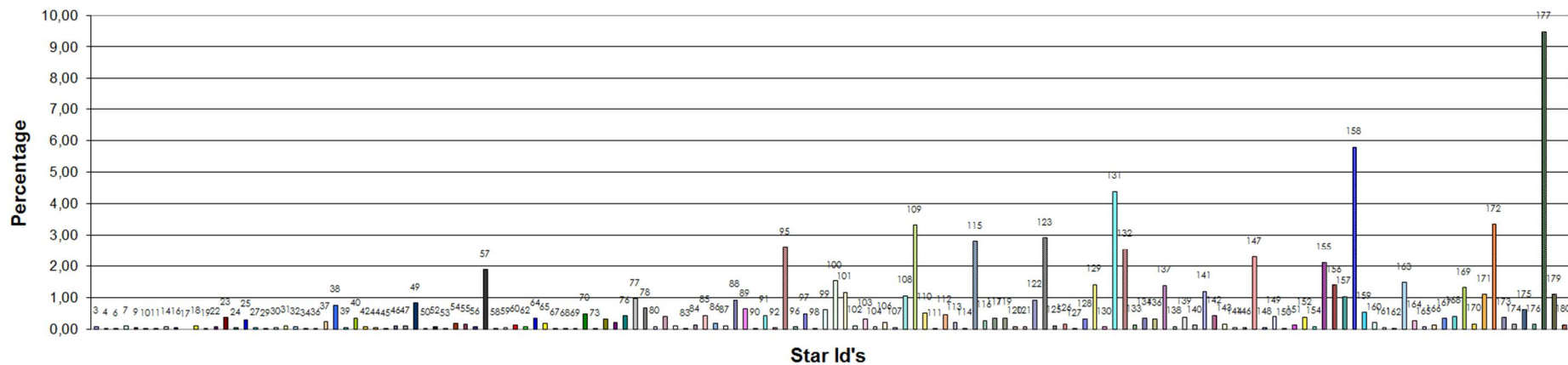
Figure 3.2-1: Statistics on stars that have been lost during the centering phase. The number above the columns corresponds to the Star ID
