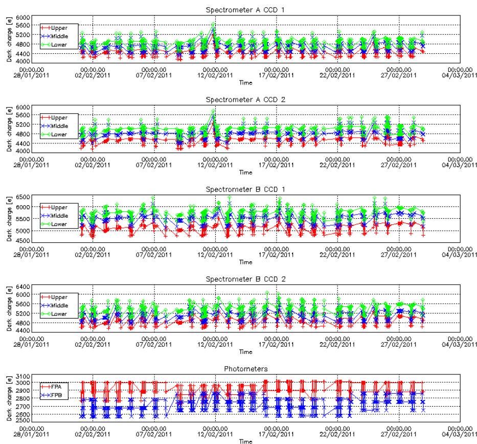
Figure 4.5-3: Mean Dark Charge of spectrometers and photometers during the reporting period
