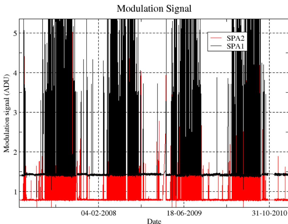
Figure 4.5-4: Modulation signal
