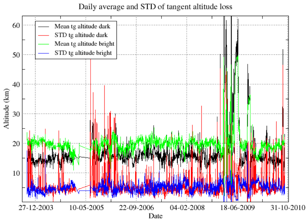
Figure 4.6-5: Daily average and STD of tangent altitude loss since the beginning of the mission
