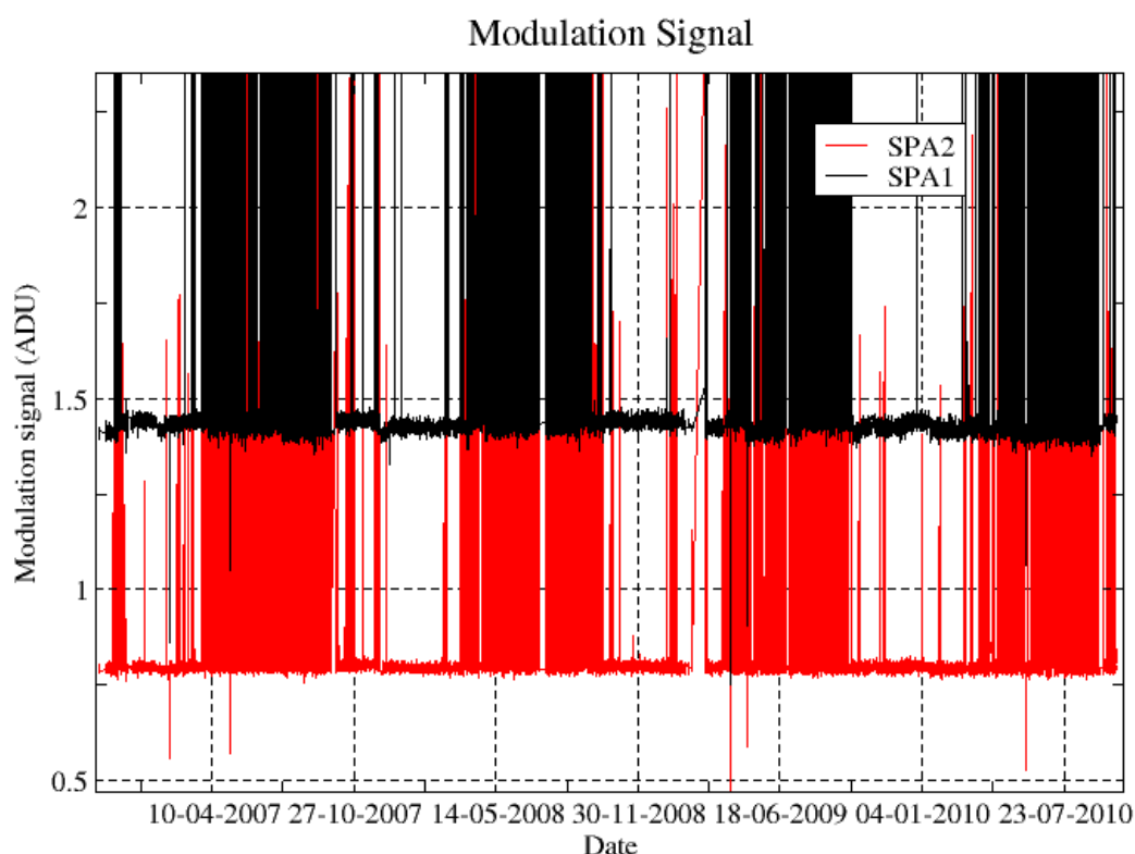
Figure 4.5-4: Modulation signal
