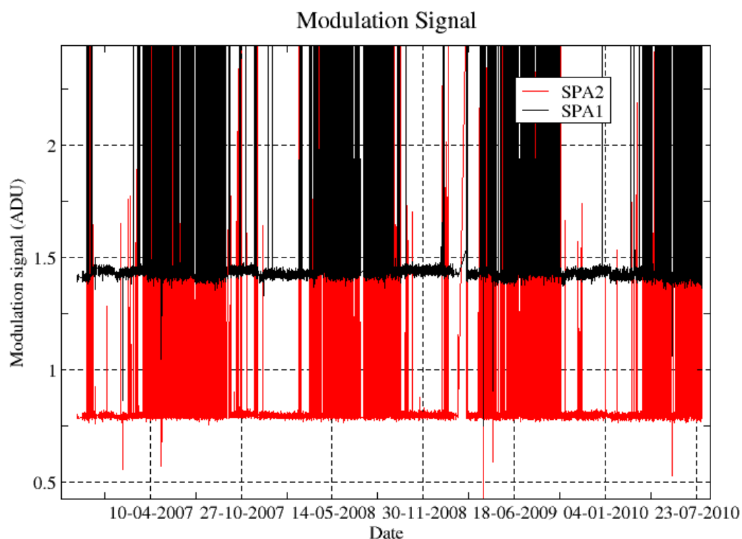
Figure 4.5-4: Modulation signal
