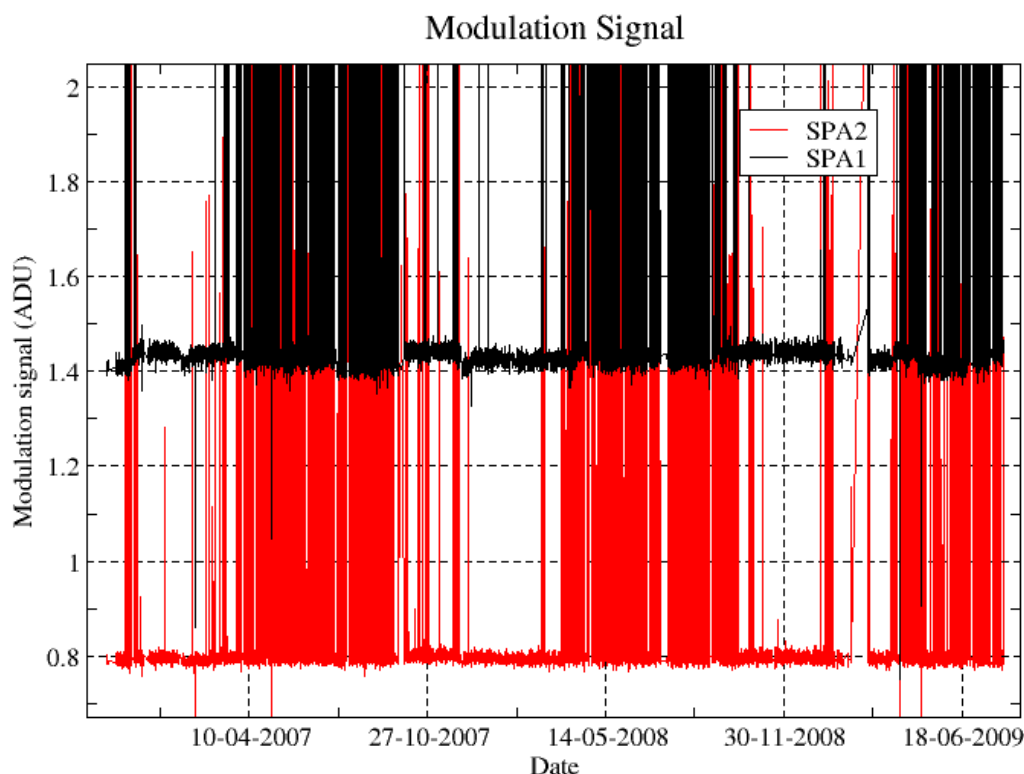
Figure 4.5-4: Modulation signal
