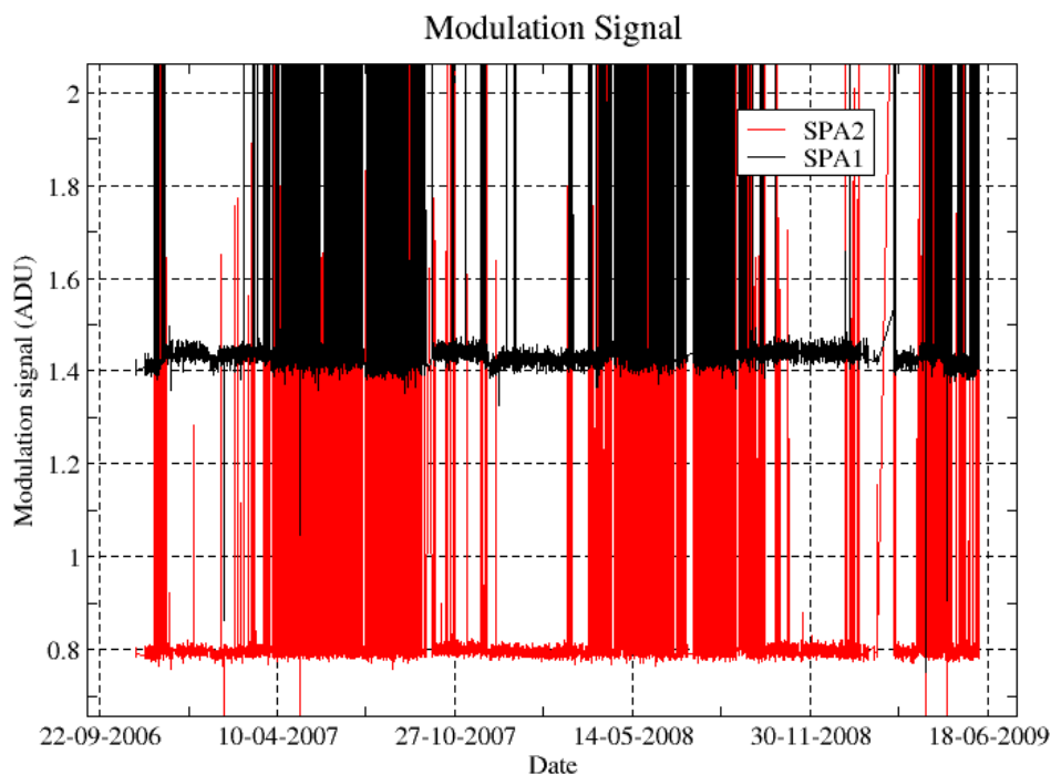
Figure 4.5-4: Modulation signal
