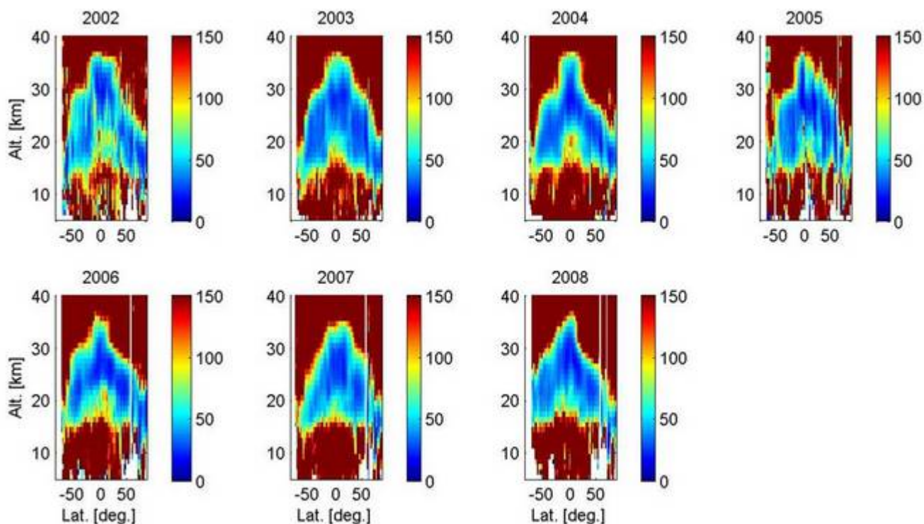
7.2-3: Zonal average of the relative variability (%) of the aerosol extinction coefficient at 500 nm for years between 2002 and 2008
