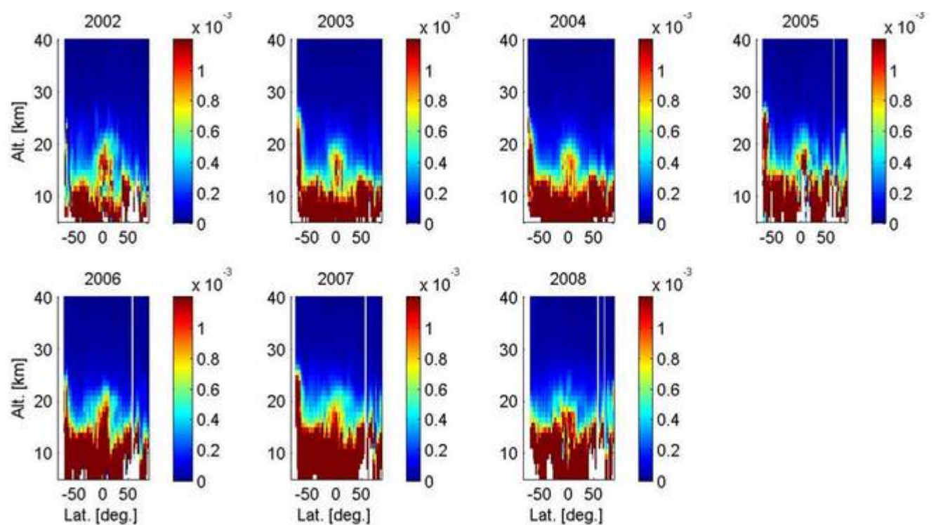
7.2-2: Zonal average of the variability of the aerosol extinction coefficient at 500 nm for years between 2002 and 2008
