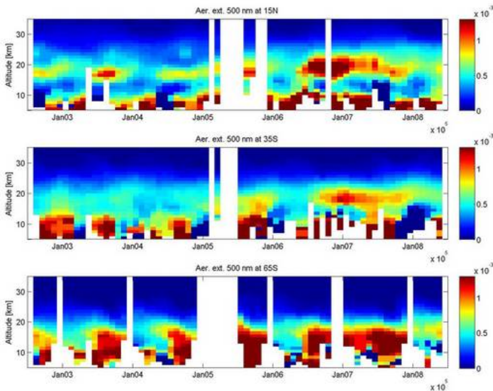
7.2-4: Time evolution of the aerosol extinction at 500 nm vs altitude at 15°N, 35°S, 65°S
