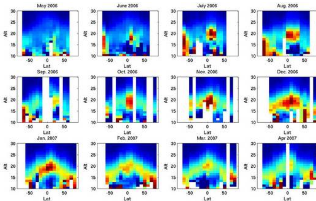
7.2-6: Monthly averages of the aerosol extinction at 500 nm vs latitude and altitude between May 2006 and April 2007
