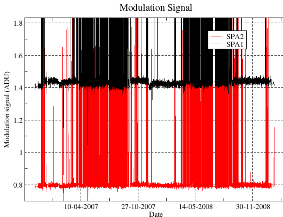
Figure 4.5-4: Modulation signal
