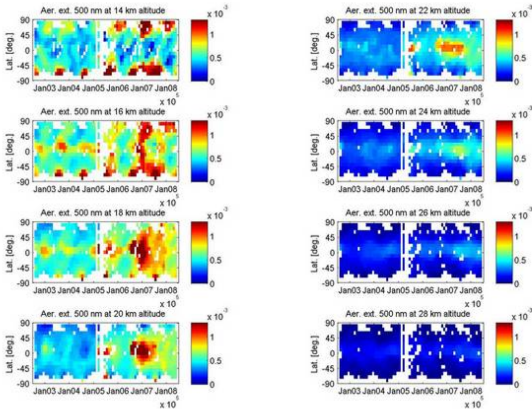
7.2-5: Time evolution of the aerosol extinction at 500 nm vs latitude at altitude levels between 14km and 28km
