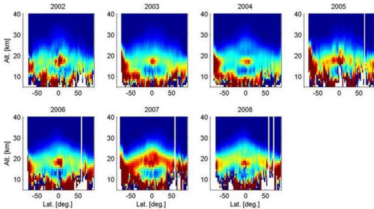
7.2-1: Yearly zonal average of the aerosol extinction at 500 nm for years between 2002 and 2008
