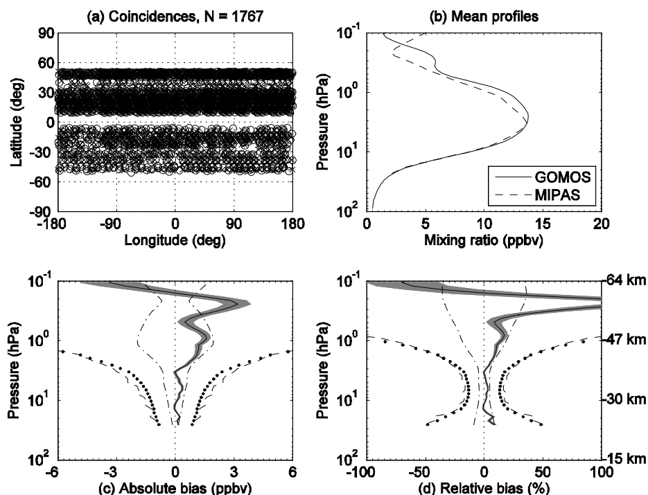
Figure 7.2-1: Case of January 2004, low-to-mid latitudes. (a) Measurement locations of GOMOS (o) and MIPAS (x). N is the number of coincident pairs. (b) Average NO 2 mixing ratios. (c) Bias (solid line), standard error of the bias (gray shading), standard deviation of the bias (dashed line), average of combined random error (dots), and average of MIPAS systematic error (dash-dot line). (d) Same as (c) but relative values as a percentage of the MIPAS mean
