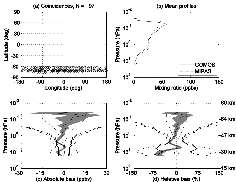
Figure 7.2-2: Same as Figure 7.2-1 for case of July 2003, polar winter latitudes.
