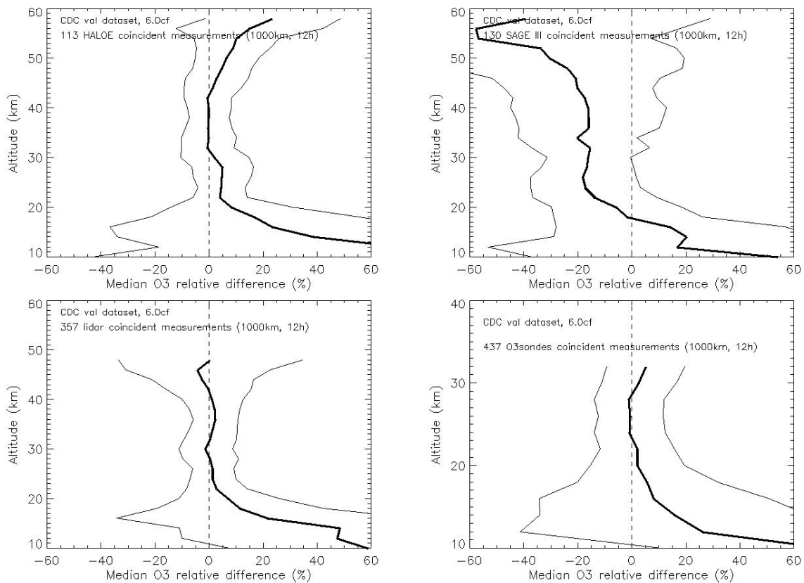
Figure 7.2-2: CDC dataset
