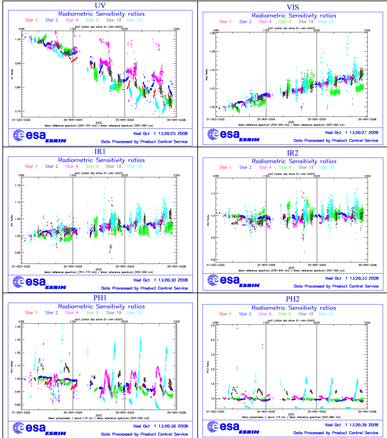
Figure 5.4-1: Radiometric sensitivity ratios since December 2002
