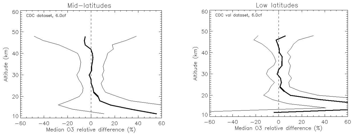
Figure 7.2-3: Comparison results for CDC dataset with lidar profiles for mid-latitude regions (left) and for low latitude regions (right)
