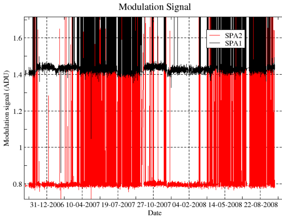
Figure 4.5-4: Modulation signal
