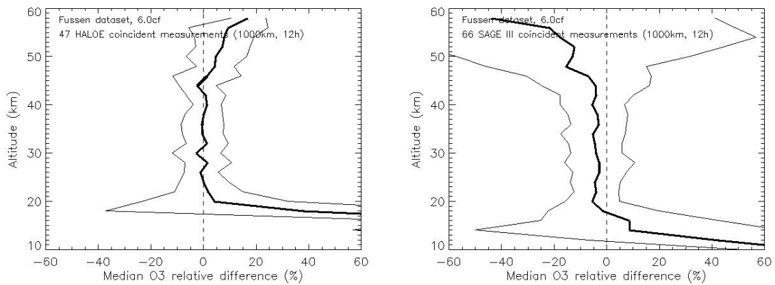
Figure 7.2-1: Fussen dataset
