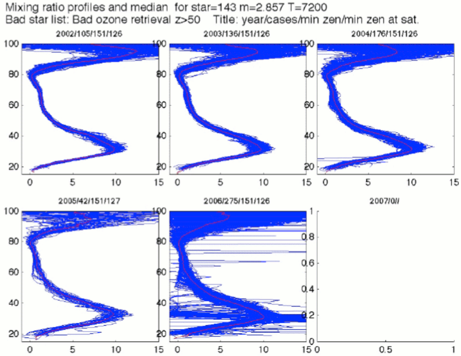
Figure 7.2-8: Same as fig. 7.2-3 for vertical profiles of O 3 mixing ratio from star 143 (T = 7200K)
