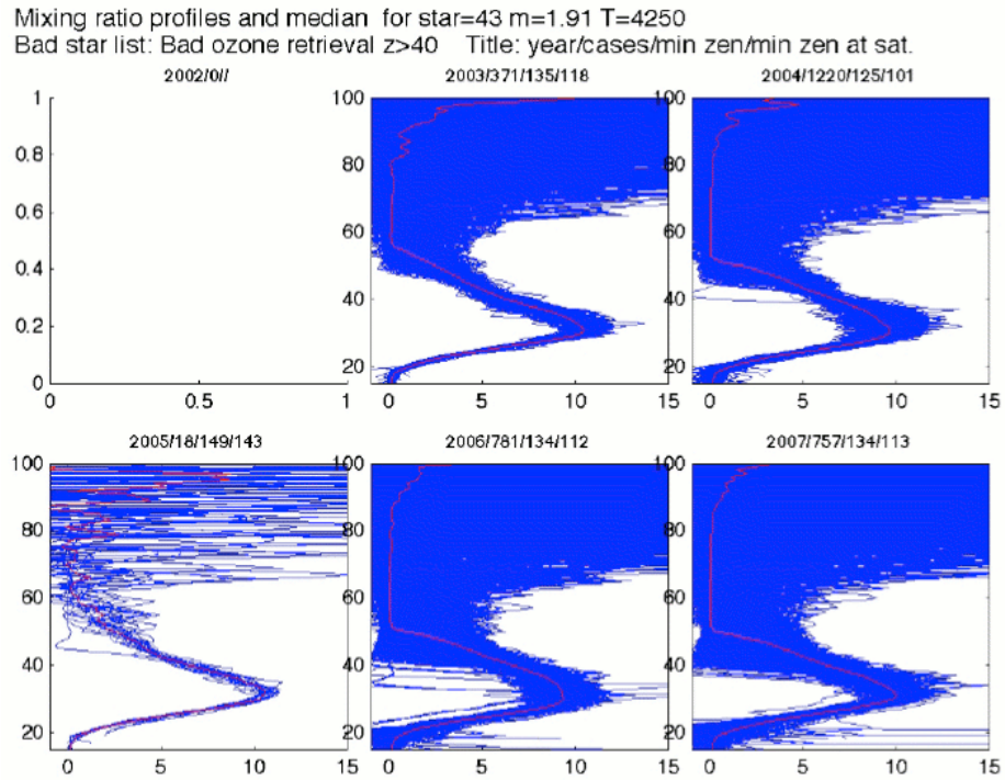
Figure 7.2-4: Same as fig. 7.2-3 for vertical profiles of O 3 mixing ratio from star 43 (T = 4250K)
