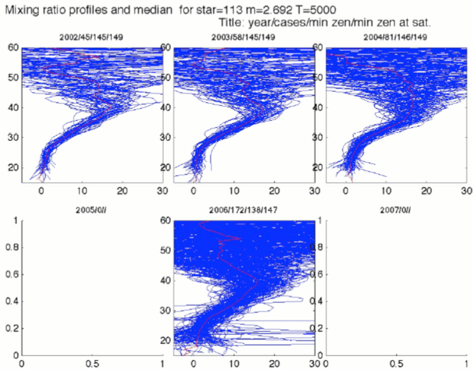
Figure 7.2-7: Same as fig. 7.2-3 for vertical profiles of NO 2 mixing ratio from star 113 (T = 5000K)
