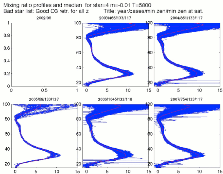
Figure 7.2-3: Vertical profiles of O 3 mixing ratio per year between 2002 and 2007 for star 4 (T = 5800K). The red line is the yearly median profile
