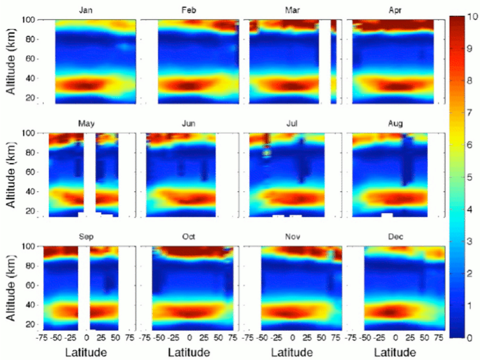
Figure 7.2-1: Monthly charts of O 3 mixing ratio in ppm (altitude vs latitude) for full dark occultations of 2003
