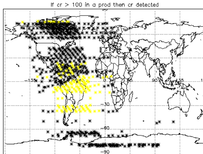
Figure 5.2-2b: Count every time a cosmic ray has been detected. When it is > 100, then cosmic rays detected (yellow in the plot)
