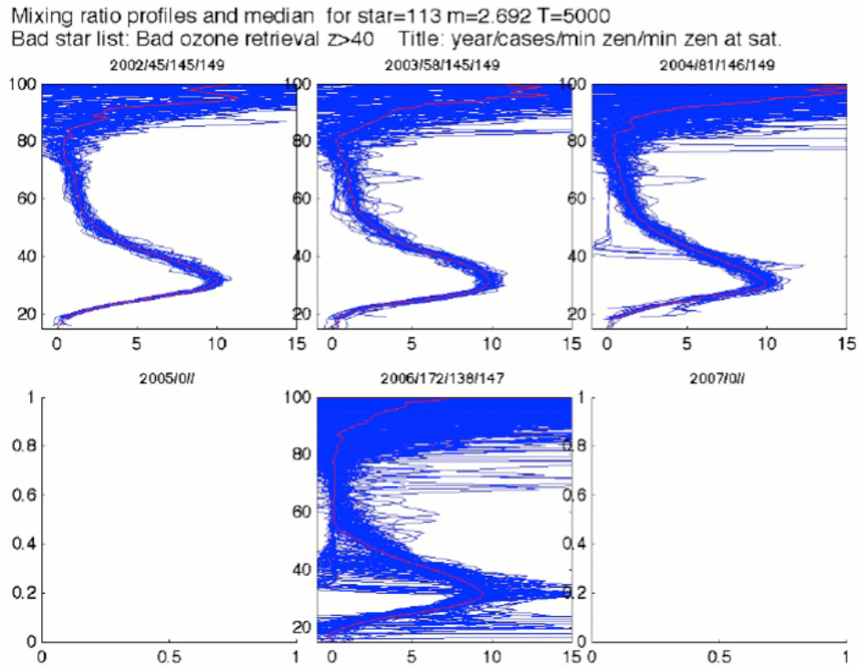
Figure 7.2-6: Same as fig. 7.2-3 for vertical profiles of O 3 mixing ratio from star 113 (T = 5000K).
