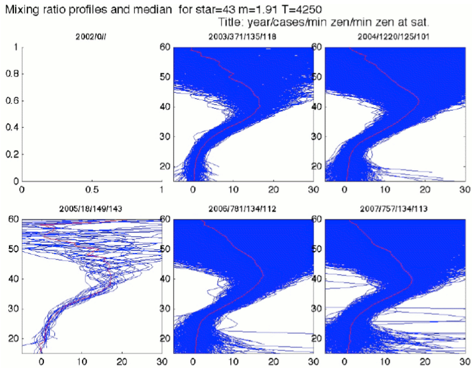
Figure 7.2-5: Same as fig. 7.2-3 for vertical profiles of NO 2 mixing ratio from star 43 (T = 4250K)
