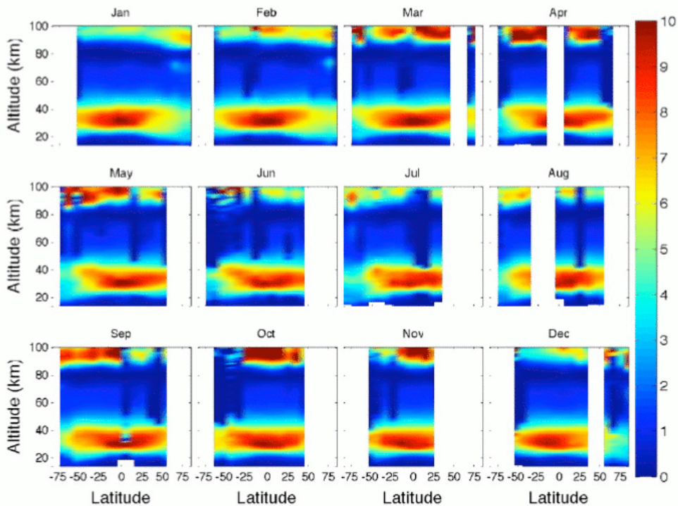
Figure 7.2-2: Same as fig. 7.2-1 for full dark occultations of 2007
