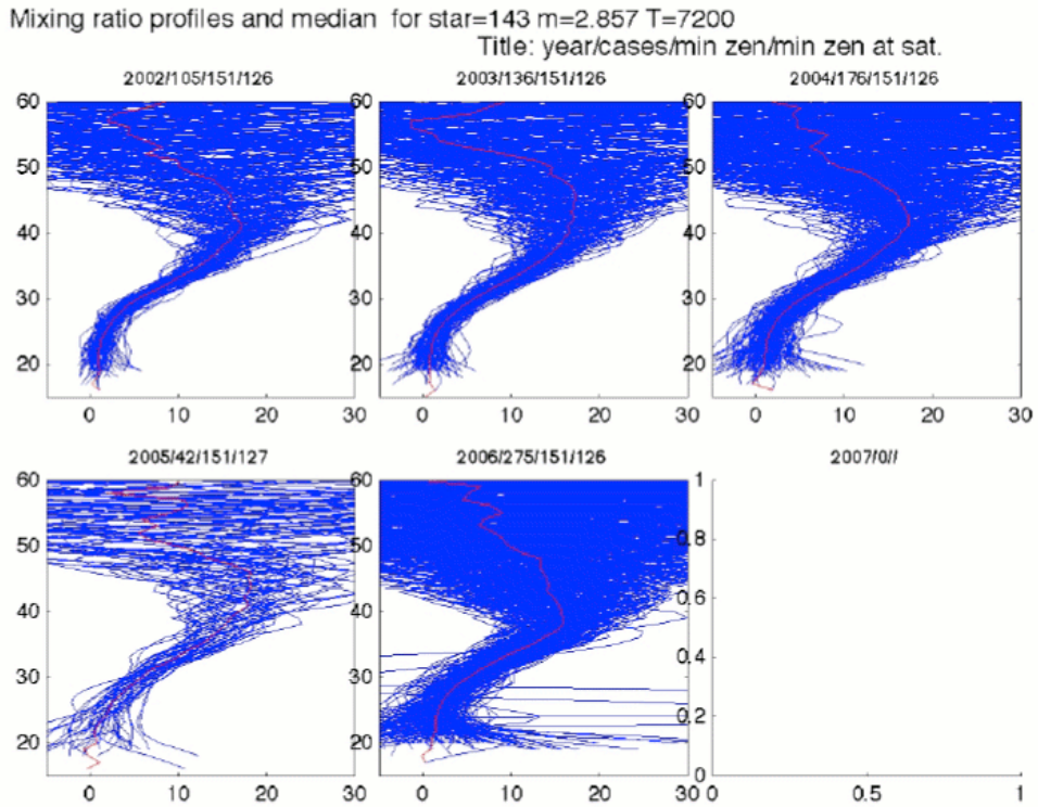
Figure 7.2-9: Same as fig. 7.2-3 for vertical profiles of NO 2 mixing ratio from star 143 (T = 7200K)
