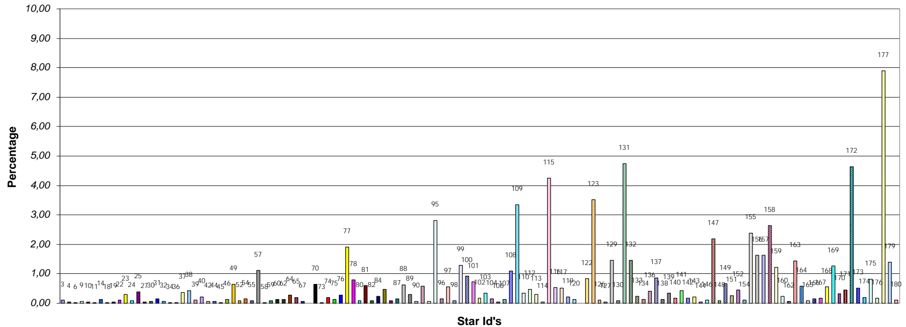
Figure 3.2-1: Statistics on stars that have been lost during the centering phase. The number above the columns correspond to the Star ID
