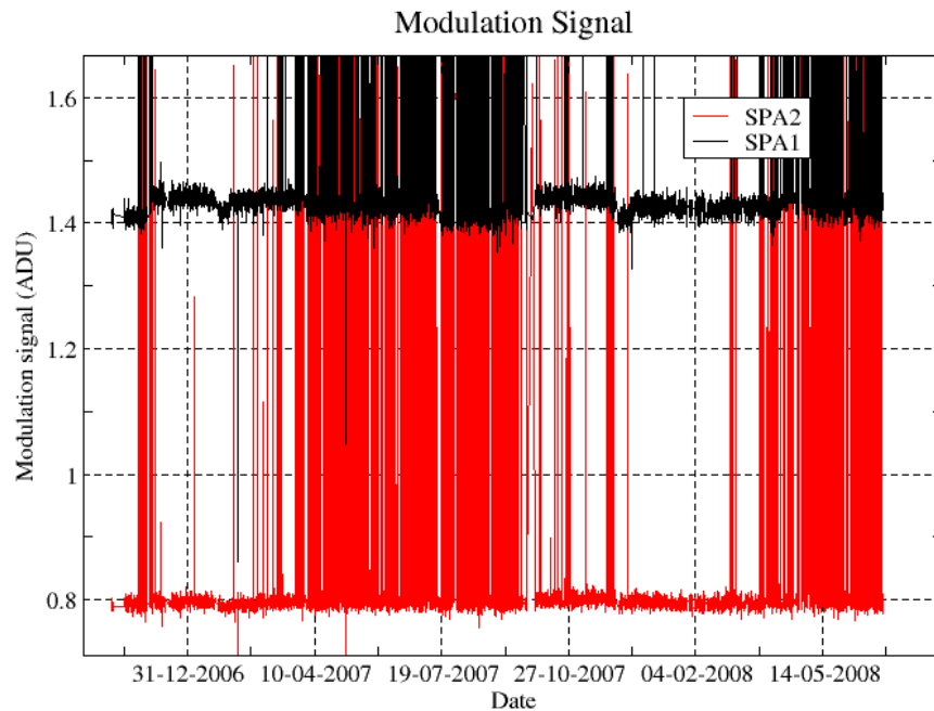
Figure 4.5-4: Modulation signal
