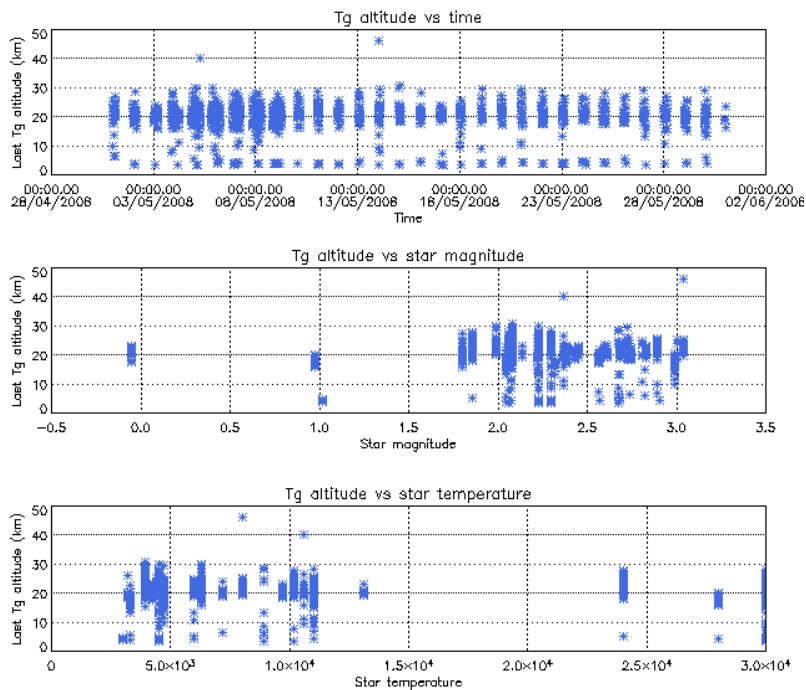
Figure 4.6-3: Last tangent altitude of the occultation (bright limb), point at which the star is lost
