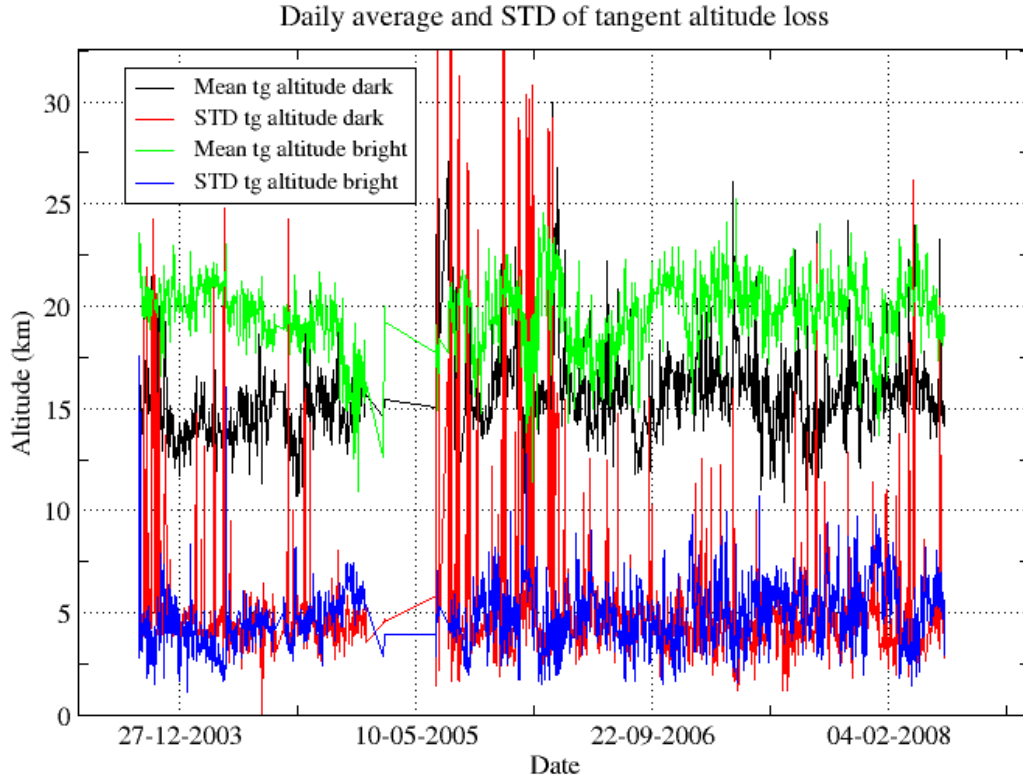
Figure 4.6-4: Daily average and STD of tangent altitude loss for the reporting period
