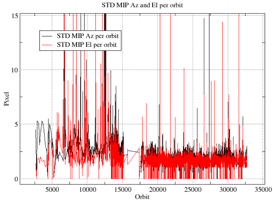
Figure 4.6-7: Standard deviation of MIP Azimuth and Elevation for some orbits since 1 st September 2002 until end of reporting period (see table 4.6-1)
