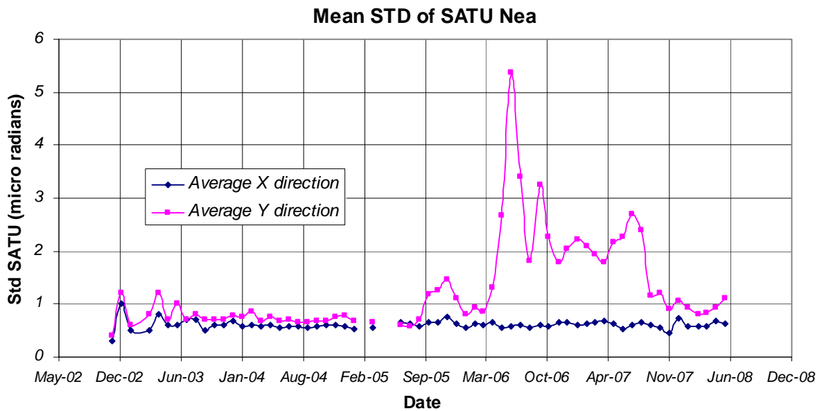
Figure 4.6-2b: Average value per month of SATU NEA STD above 105 km
