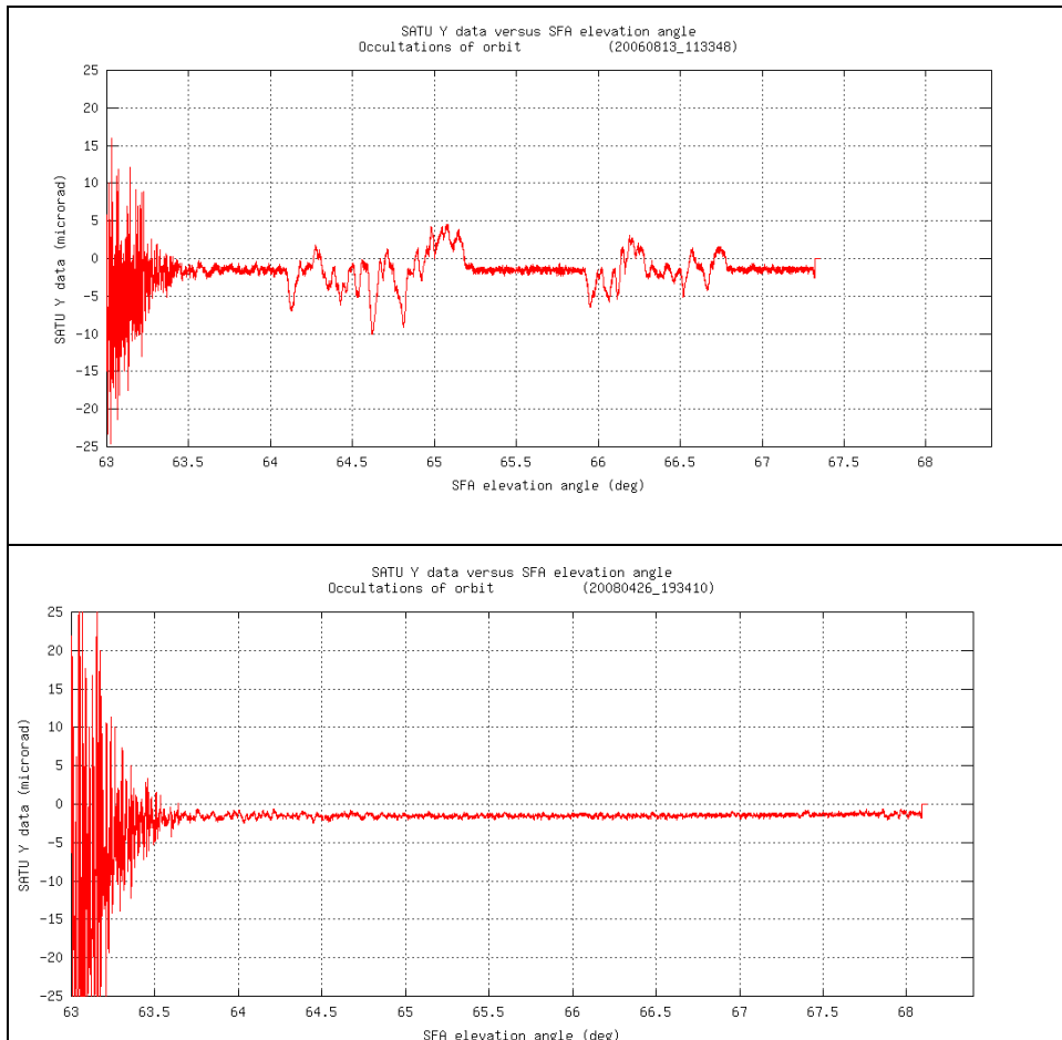
Figure 4.6-1a: SATU with anomaly (upper plot) and without anomaly (lower plot)
