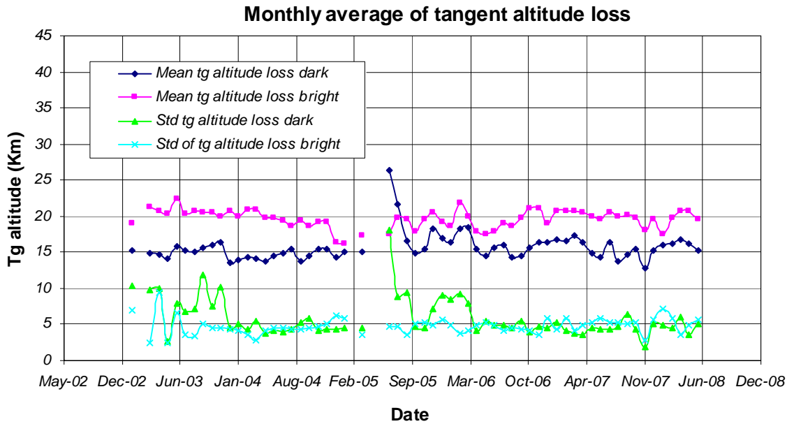
Figure 4.6-5: Monthly mean tangent altitude (and STD) at which the star is lost since January 2003
